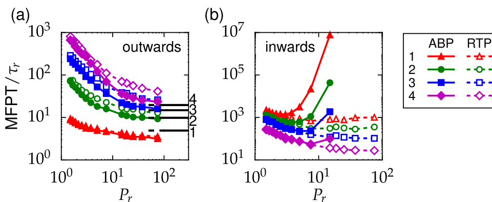
Figure 5. MFPT versus persistence number P_r , for the square maze in the outwards (a) and inwards case (b). Symbols refer to simulation data. They are connected by lines to guide the eyes. Error bars are smaller than symbols. In (a) the black horizontal lines show theoretical predictions obtained from Eq. (6) using \theta_0 = \pi , \theta_1 = 0 , and \theta_2 = 2\pi . The adjacent numbers refer to the opening index.
