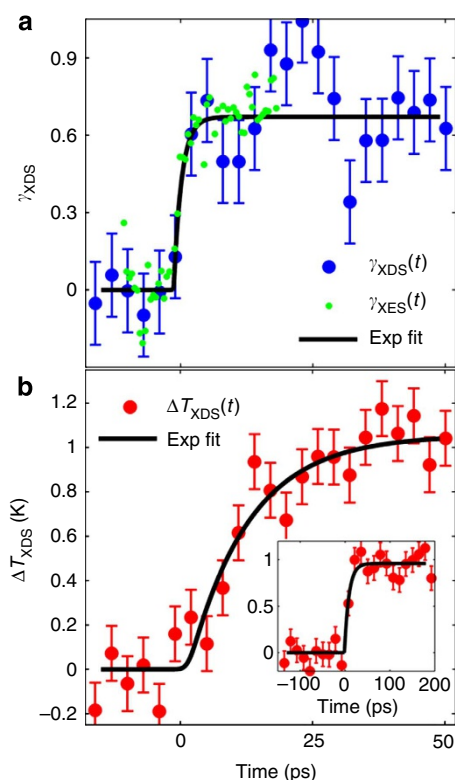
Figure 6 | Ultrafast XDS kinetics. (a) \gamma_{\text{XDS}}(t) (blue dots) and \gamma_{\text{XES}}(t) (green dots) as a function of pump-probe time delay. The single-exponential fits of \gamma_{\text{XDS}}(t) is indicated by the black line. (b) \Delta T(t) kinetics (red dots), with its single-exponential fit (black line). The error bars six indicate the s.d. of the data points.
