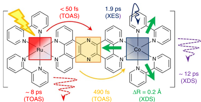
Figure 8 | Non-equilibrated ET across the photoexcited [^1\text{Ru}^{\text{II}}=^1\text{Co}^{\text{III}}] dyad. The schematic summarizes the fundamental timescales, as obtained from TOAS and combined XES-XDS at the SACLA XFEL facility.
