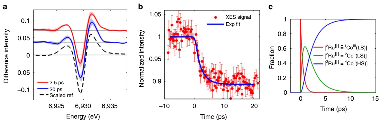
Figure 4 | Ultrafast X-ray emission spectroscopy. (a) Co K\alpha_1 \Delta S_{\text{XES}}(t) at 2.5 (red) and 20 ps (blue) pump-probe delay. The shaded areas indicate the uncertainty level. The dashed black curve is the simulated reference for a {}^1\text{Co}^{\text{III}}(\text{LS}) \rightarrow {}^4\text{Co}^{\text{II}}(\text{HS}) conversion, scaled to the 20 ps trace. (b) Kinetic trace at 6.93 keV (red dots) and single-exponential fit with a 1.9 ps lifetime, broadened by a 520 \pm 410 fs XFEL IRF (blue line). The error bars indicate the s.e. of each data point. (c) Time evolution for the fractions of [{}^2\text{Ru}^{\text{III}}(=\bullet){}^1\text{Co}^{\text{III}}(\text{LS})] (red), [{}^2\text{Ru}^{\text{III}}={}^2\text{Co}^{\text{II}}(\text{LS})] (green) and [{}^2\text{Ru}^{\text{III}}={}^4\text{Co}^{\text{II}}(\text{HS})] (blue) as monitored by the combination of femtosecond TOAS and XES, where the initial fraction of [{}^2\text{Ru}^{\text{III}}(=\bullet){}^1\text{Co}^{\text{III}}(\text{LS})] was renormalized to 1.
