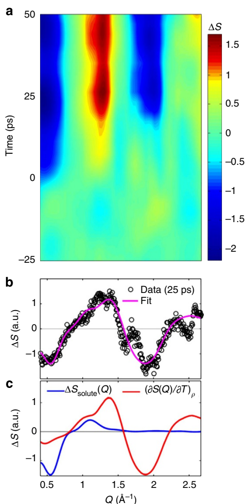
Figure 5 | Ultrafast X-ray diffuse scattering. (a) Median filtered \Delta S_{\text{XDS}}(Q,t) . (b) Experimental (black dots) and fitted (purple line) \Delta S_{\text{XDS}}(Q, 25 \text{ ps}) . (c) Contributions from the solute (blue) and from the solvent (red).
