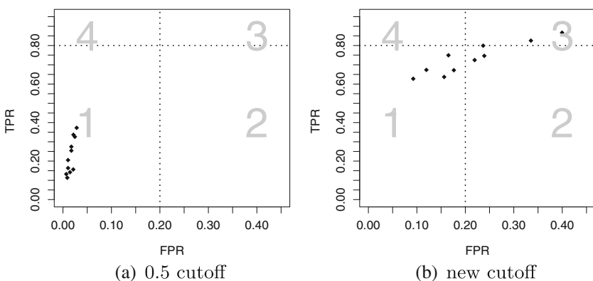
Fig. 4 Plots of accuracy for two different cutoffs evaluating vulnerability for three years ahead using the same underlying model assuming normal log incomes. Best predictions lie in the 4th quadrant, worst predictions in the 2nd quadrant
