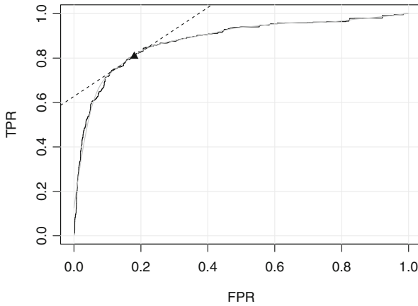
Fig. 1 ROC curve based on SOEP data, year 1995. The solid black (gray) line represents the (smoothed curve of) TPR/FPR-combinations for each possible cutoff. Using the targeting differential as targeting mechanism, the dashed tangential line determines the optimal TPR/FPR combination that is marked with a triangle. Illustration is based on Klasen and Lange (2016)
