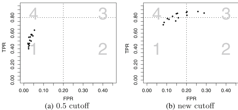
Fig. 3 Plots of accuracy for two different cutoffs and same underlying model assuming normal log incomes. Best predictions lie in the 4th quadrant, worst predictions in the 2nd quadrant
