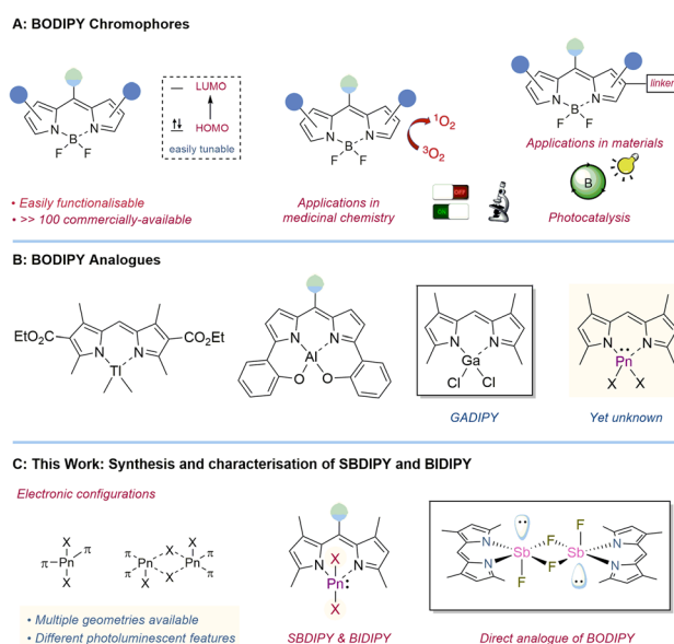
Fig. 1 Context of the work. (A) BODIPY chromophores (B) previous heavier BODIPY analogues. (C) Synthesis and characterisation of SBDIPY and BIDIPY.
