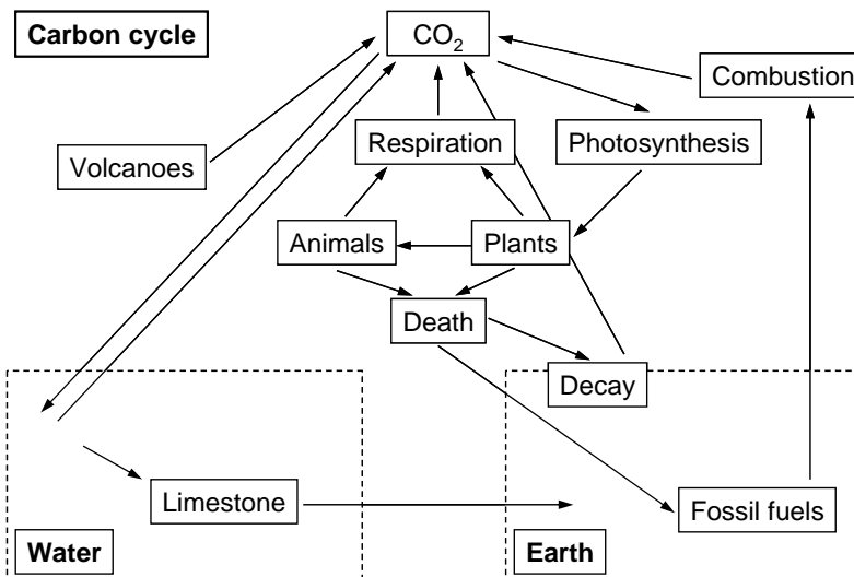
Fig. 2 Schema of global carbon cycle
