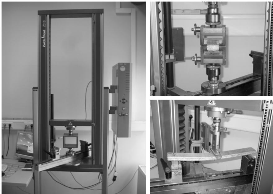
Fig. 13 Universal test machine (Zwick/Roell ZO10, 10 kN test load, Zwick/Roell, Ulm, Germany) in the "Biotechnikum" (pilot plant station) at the Institute of Forest Botany in Göttingen used for determining mechanical-technological properties of wood-based panels and of solid wood. A. Test equipment for determining surface strength of wood-based panels. B. Test equipment to determine internal bond strength of wood composites and of solid wood. C. Test equipment for determining bending strength and modulus of elasticity for composites and solid wood. Forces are applied by the test machine to samples of defined sizes until these break. Corresponding values are measured and transferred to a computer where they are analysed by a special software
