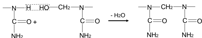
Fig. 8 Condensation reactions of urea and formaldehyde to urea-formaldehyde resins (see Habenicht 1997, Christjanson et al. 2006)
