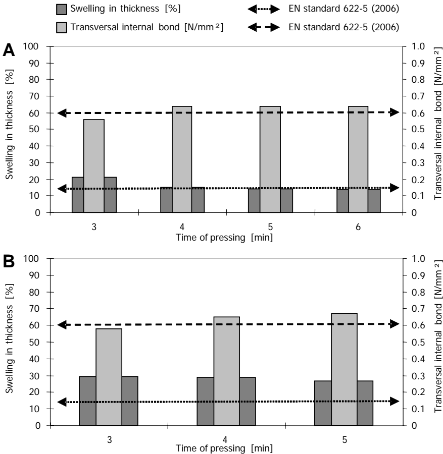
Fig. 3 Swelling in thickness after 24 h in water and transversal internal bond strength of medium density fibreboard (MDF). A. MDF produced with 100% mechanically–enzymatically decomposed potato-pulp, 2% keying agent, and 2% hydrophobic wax (relative to absolute dry fibre). B. MDF produced with a 1:1 mixture of urea-formaldehyde resin and mechanically-enzymatically decomposed potato-pulp (relative to absolute dry fibre). Properties were tested on the basis of European standard EN 622-5 (2006)
