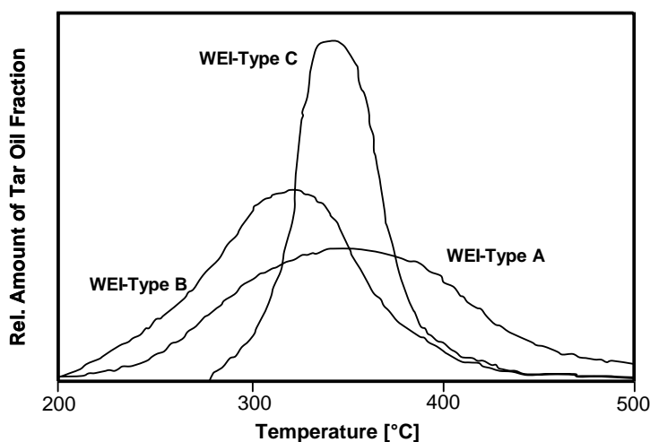
Fig. 1 Distillation curves of WEI tar oil types (Poducer information Rütgers Organics, Mannheim)
