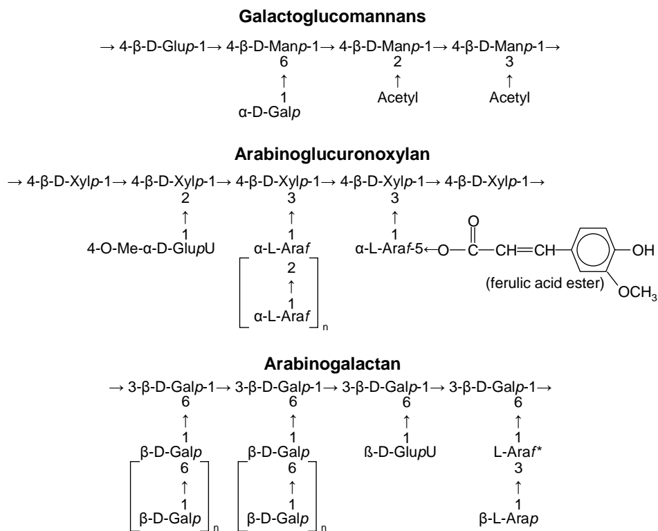
Fig. 6. Representative structures of the main hemicelluloses from softwood (for abbreviations and chemical structures see Fig. 4; * denotes that at this position either \alpha -L-Araf or \beta -L-Araf might be inserted)
