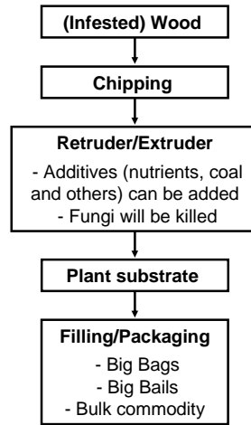
Fig. 3 Schematic diagram of the peat substitute production. The Retrunder ® process has originally been developed for bare wood but can also be performed with infested wood
