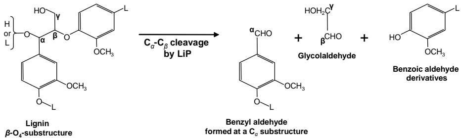
Fig. 3 C α -C β cleavage by lignin peroxidase in a representative non-phenolic lignin-substructure; L = lignin (adapted from Hammel et al. 1993)
