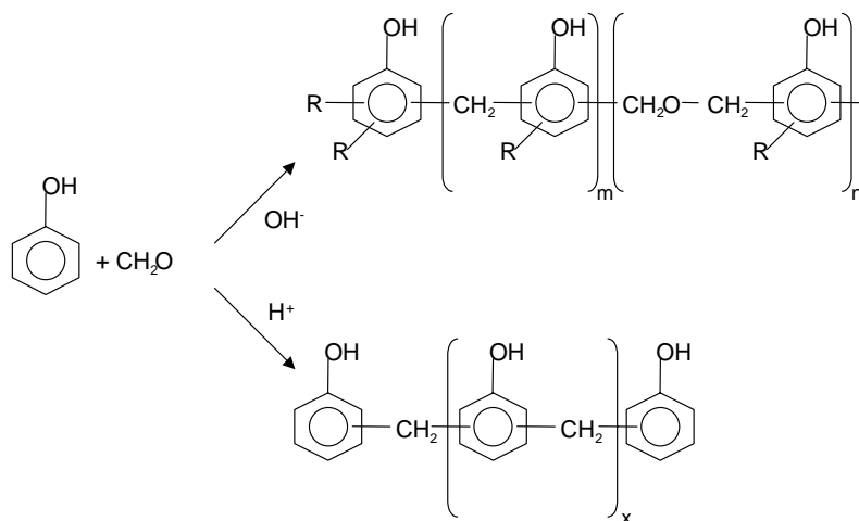
Fig. 10 Polycondensation reactions of phenol-formaldehyde resins – resol is formed when \text{OH}^- is used as catalysator (top), novalak with \text{H}^+ as catalysator (bottom)
