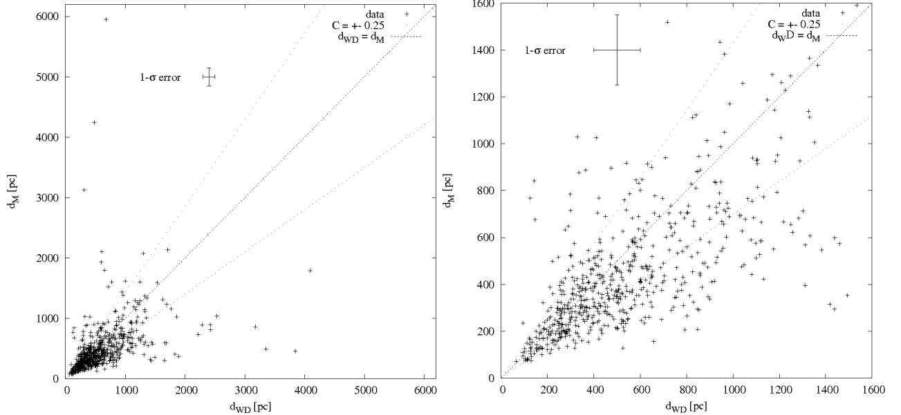
Fig. 6. Distribution of the derived distances of the stellar components of our systems; the diagonal is the ideal for physical binaries. The dotted curves span a tolerance fan for C = 0.25 . Left : note that for very far away – and thus rather faint – objects with a distance of more than \approx 1000 pc the distance for the respective binary mate is typically very different. This is due to the weak spectroscopic features of the distant stars and the low spectral resolution. Right : same as left but zoomed in.
