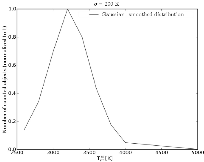
Fig. 8. T_{\text{eff}}^{\text{M}} function; the cutoff at 2600 K towards lower temperatures is due to our lack of cooler models. The peak at 3200 K is probably generated by SDSS selection effects and does not reflect the true M dwarf population. The tail towards T_{\text{eff}}^{\text{M}} > 3800 K is caused by 4 objects with insecure fit at T_{\text{eff}}^{\text{M}} = 4000 K and the Gaussian decay.
