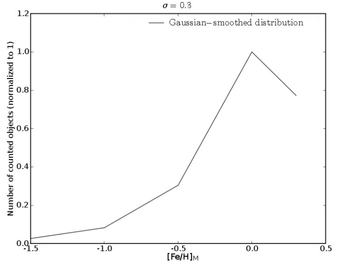
Fig. 13. Metallicities of the M stars in our sample, normalized to 1; the plot shows a distinct peak at [\text{Fe}/\text{H}]_M = 0 . PHOENIX models for [\text{Fe}/\text{H}]_M > 0.3 were not available. Among the 70 candidates for a VLMO, there is only J1323+3018 showing a metallicity >0 .
