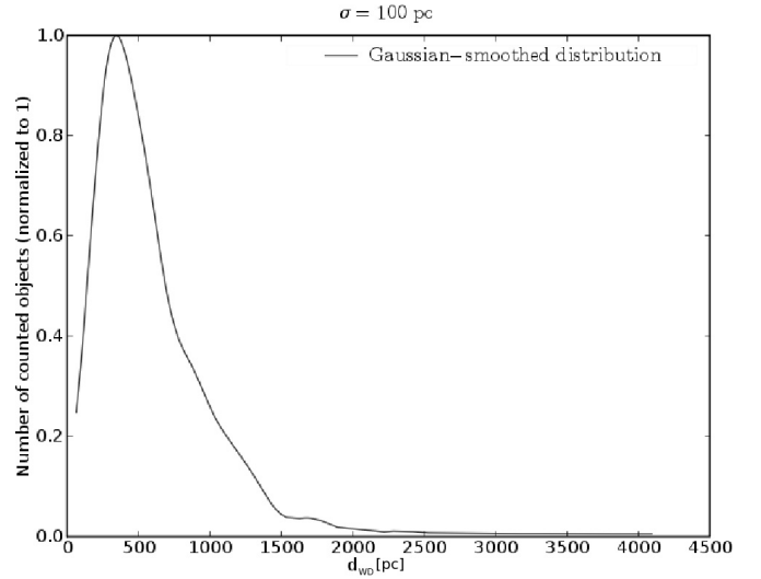
Fig. 9. The distribution of the WD distances in our sample is a consequence of the restricted magnitude range of the SDSS. It has its maximum at 354 pc.
