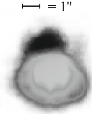
Fig. 14. As an example for one of the 41 optically resolved binaries with further treatment, we show the SDSS image of J1127–0028. The image resolution is 0.025''/\text{pixel} . In this grayscale image, the red companion is set black while the larger and brighter spot is the white dwarf.
