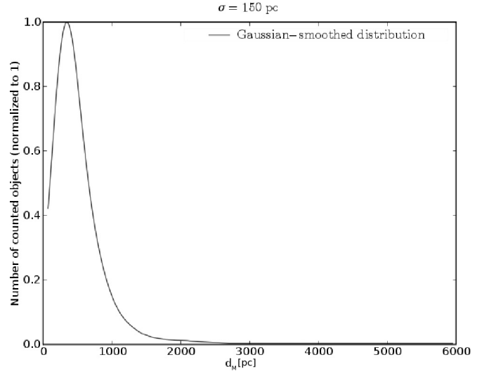
Fig. 10. The distribution of the M star distances in our sample is a consequence of the restricted magnitude range of the SDSS. Its maximum is at 334 pc.
