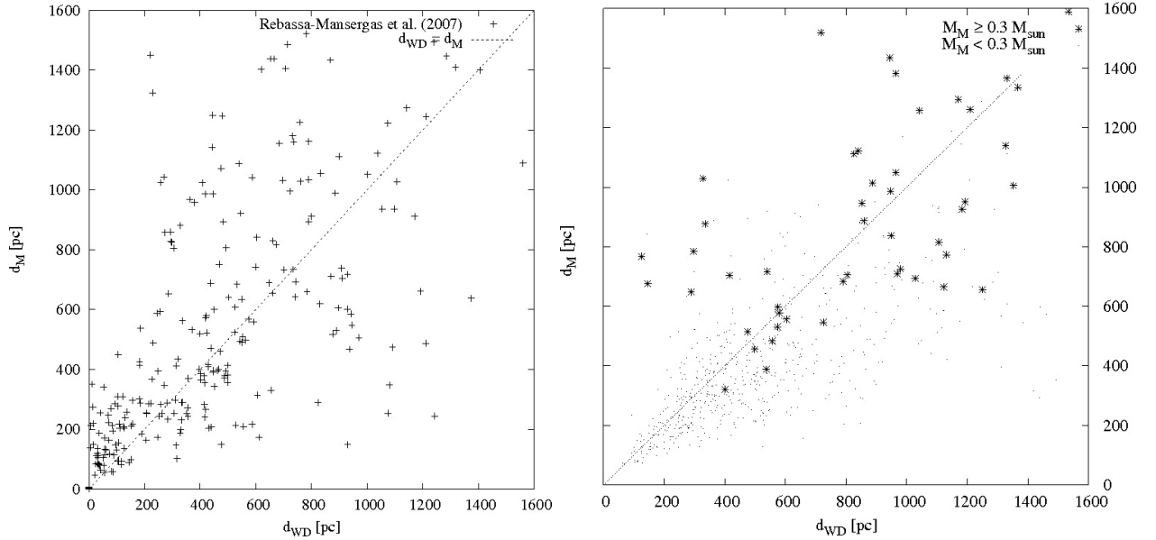
Fig. 16. Left: distribution of the derived distances of the stellar components from Rebassa-Mansergas et al. (2007) ; in contrast to our results, their binaries tend to have a larger value for d_M than for d_{WD} . Right: for M stars with masses \geq 0.3 M_{\odot} there is no tendency of d_M < d_{WD} in our data.
