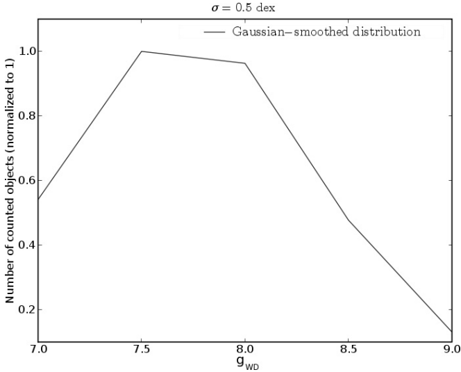
Fig. 11. Distribution of the WD surface gravities.
