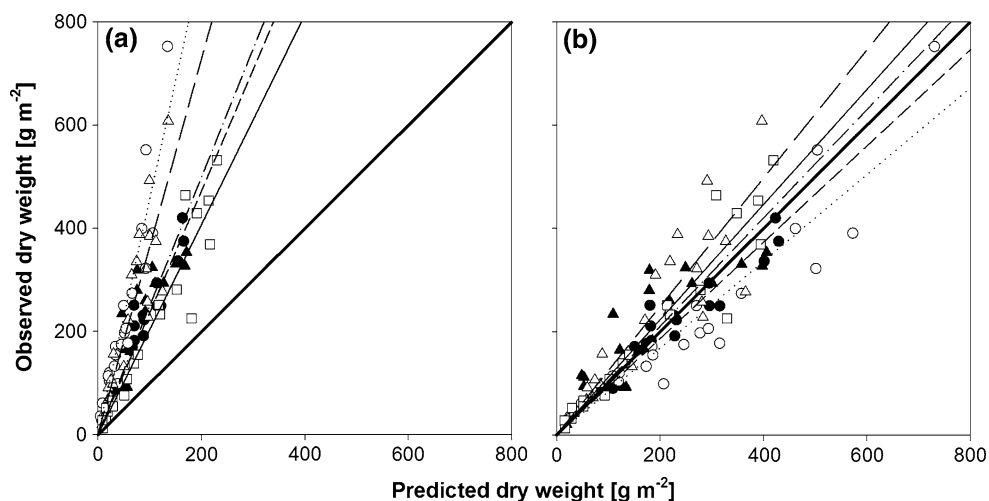
Fig. 2 Modelled vs. observed dry weights on clearcuts for (filled circle) A. capillaris , (filled triangle) D. flexuosa , (open triangle) D. purpurea , (open circle) E. angustifolium and (open square) R. idaeus ; a using the uncorrected PhytoCalc model, b using the model corrected by multiplication with CF^2 ; Regression lines are given for each species ( A. capillaris : short dash; D. flexuosa : dash dot; D. purpurea :
