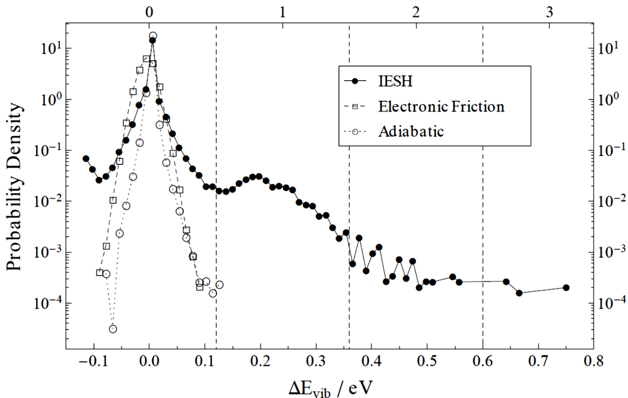
FIG. 2: Theoretical calculations of vibrational probability density as a function of the change in vibrational energy, \Delta E_{\text{vib}} , for E_i=0.63 eV and T_s=1000 K. The zero of the x -axis in this figure represents the zero point energy level with 0.12 eV of vibrational energy. Hence, the classical calculation allows loss of vibrational energy resulting in values below the zero point level. Such trajectories are binned as v=0 . Results are shown for adiabatic dynamics (no surface hopping, open circles), electronic friction (open squares), and for IESH (solid circles). Vertical dashed lines show the binning regions for each vibrational state ( v=0, 1, 2 and 3 ), which are indicated on the upper x -axis. IESH predicts a much larger vibrational excitation probability than does electronic friction theory or the adiabatic treatment. Note the logarithmic scale.
