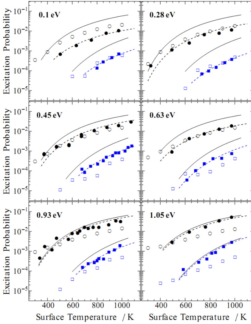
FIG. 3: Excitation probabilities for NO/Au(111) as a function of surface temperature, T_s , for six different incidence energies of translation, E_i . Experiment (filled) and IESH theory (empty): NO( v=0 \rightarrow 1 ) – black circles, and NO( v=0 \rightarrow 2 ) – blue squares. Arrhenius fits to the experimental points are shown as dashed lines. Thermal limits are shown as solid lines.
