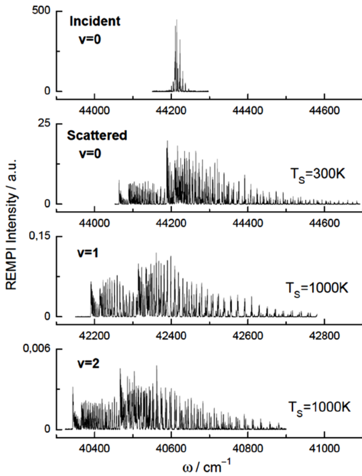
10 FIG. 1: REMPI spectra for incident and scattered NO at E_i=0.63\text{eV} corrected for difference in laser power and MCP gain. The NO( v=0,1,2 ) are probed via the \gamma_{00} , \gamma_{01} and \gamma_{02} , bands, respectively. The incident beam is rotationally cold, with significant population in only a few quantum states. The molecules undergo significant rotational and vibrational excitation in the surface scattering process.
