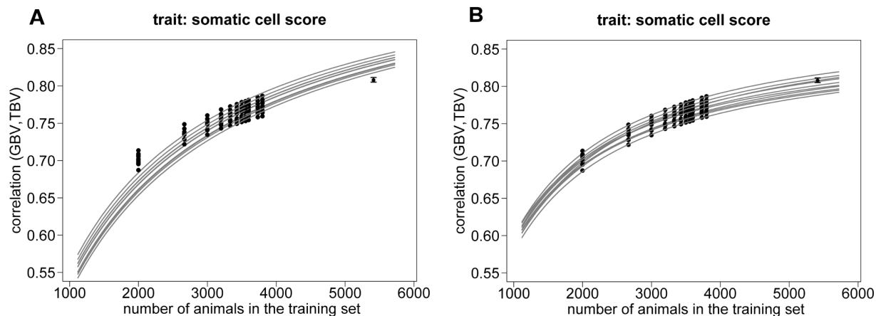
Figure 7. Predicted and empirical values of r_{GBV, TBV} when extrapolating the accuracy. Empirical values of r_{GBV, TBV} (black dots) of the ten replicates with different k-fold scenarios using 4'000 individuals and of the 20-fold runs of the fifty replicates using 5'698 Holstein-Friesian animals in total. Expected values (grey lines) use the number of M_e derived with a Maximum-Likelihood approach in the original equation of Daetwyler et al. (2010) (D1, Figure 7A) and in the modified equation of Daetwyler et al. (2010) (D2, Figure 7B). doi:10.1371/journal.pone.0081046.g007
