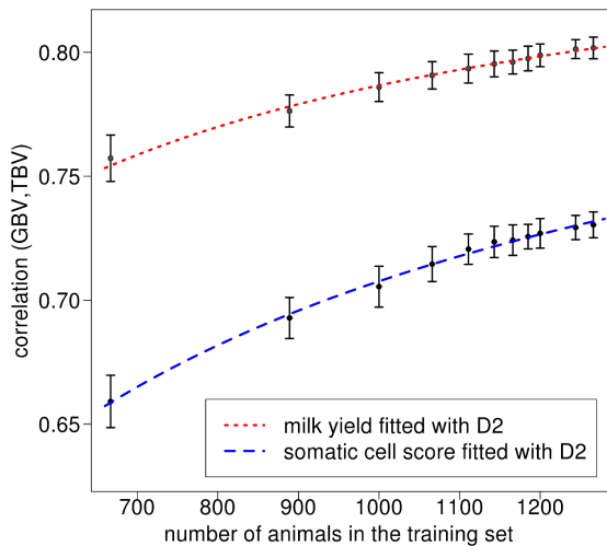
Figure 5. Empirical values and expected values of r_{GBV, TBV} for milk yield and somatic cell score in Brown-Swiss. Empirical values of r_{GBV, TBV} and expected values using the number of M_e for the Brown Swiss data set derived with a Maximum-Likelihood approach in the modified equation of Daetwyler et al. (2010) (D2). For the empirical values of milk yield and somatic cell score in the Brown Swiss data set, the mean and the standard deviation over the 50 replicates in each k-fold scenario are shown. doi:10.1371/journal.pone.0081046.g005
