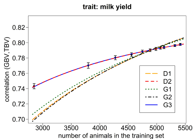
Figure 1. Empirical values and expected values of r_{GBV, TBV} for milk yield in Holstein-Friesian data. Empirical values of r_{GBV, TBV} and expected values using the number of M_e derived with a Maximum-Likelihood approach for the Holstein-Friesian data set in the original equation of Daetwyler et al. (2010) (D1) as well as in a modified form (D2) and in the equation of Goddard et al. (2011) without (G1) and with (G2) the proposed correction factor, respectively, and with the factor b not further determined (G3). For the empirical values, the mean and the standard deviation over the 50 replicates in each k-fold scenario of the Holstein-Friesian data set are shown. doi:10.1371/journal.pone.0081046.g001
