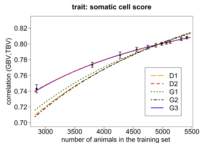
Figure 2. Empirical values and expected values of r_{GBV, TBV} for somatic cell score in Holstein-Friesian data. Empirical values of r_{GBV, TBV} and expected values using the number of M_e derived with a Maximum-Likelihood approach for the Holstein-Friesian data set in the original equation of Daetwyler et al. (2010) (D1) as well as in a modified form (D2) and in the equation of Goddard et al. (2011) without (G1) and with (G2) the proposed correction factor, respectively, and with the factor b not further determined (G3). For the empirical values, the mean and the standard deviation over the 50 replicates in each k-fold scenario of the Holstein-Friesian data set are shown. doi:10.1371/journal.pone.0081046.g002
