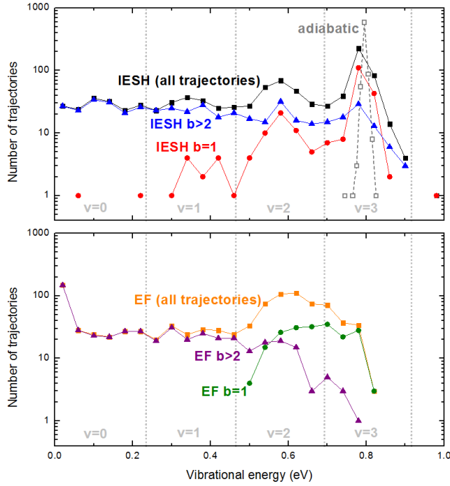
FIG. 9. The top figure shows classical vibrational energy distributions for IESH (black squares), IESH after selection of single-bounce trajectories ( b=1 , red circles), IESH after selection of multi-bounce trajectories ( b>2 , blue triangles), and for an adiabatic simulation (gray open squares). The bottom figure shows similar distributions for EF simulations (all trajectories: orange squares; b=1 : green circles; b>2 : purple triangles). The bins for quantized vibrational states v=0,1,2,3 are indicated by the vertical dotted lines. The initial vibrational energy was set to E_{\text{vib}}^0=0.80\text{eV} , corresponding to v=3 . The incidence translational energy is E_i=0.4\text{eV} . For both IESH and EF simulations, a number of 1000 trajectories was simulated. We find that vibrational relaxation is insignificant for the adiabatic simulation, whereas both IESH and EF predict substantial relaxation. Selecting only single-bounce or only multi-bounce trajectories has a drastic influence on the resulting vibrational energy distributions. For EF, it completely suppresses the relaxation into v=1 and v=0 .
