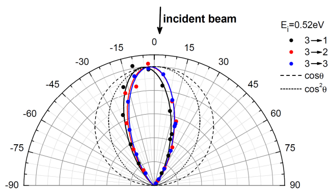
FIG. 2. Experimentally observed angular distributions for vibrational channels 3 \rightarrow 1, 2, 3 recorded at an incidence energy of E_i = 0.52 \text{ eV} . The solid lines are \cos^m(\theta - \theta_0) fits to the experimental data, with exponents m = 8.8 - 9.5 . The dashed lines are \cos\theta and \cos^2\theta distributions, the two limiting cases of angular distributions expected for a trapping-desorption mechanism under our conditions. 23 The observation of narrow angular distributions indicates that the collisions happen in a direct single-bounce mechanism.
