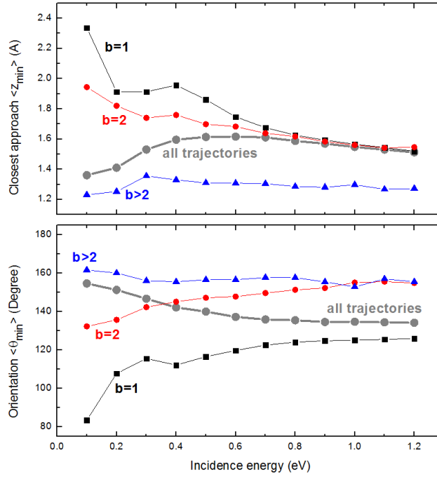
FIG. 7. Coordinates at closest approach, evaluated for all (big gray circles), single (black squares), double (red circles) and multiple (blue triangles) bounce trajectories. Top panel: The average minimal z value, \langle z_{\min} \rangle . Bottom panel: The average angle of the internuclear axis ( O \rightarrow N ) with the z -axis at the instant of closest approach, \langle \theta_{\min} \rangle , where 0^\circ , 180^\circ correspond to perfect O , N down orientation. For single and double-bounce trajectories, \langle z_{\min} \rangle decreases as the incidence energy is increased, in accordance with expectation. For multi-bounce trajectories, \langle z_{\min} \rangle is nearly constant, and very small. The overall trend mostly results from the changing fractions of single, double and multi-bounce trajectories. Similar conclusions apply for the orientation at closest approach, where favored N -down orientation with \langle \theta_{\min} \rangle near 160^\circ is found for multi-bounce trajectories over the full range of incidence energies.
