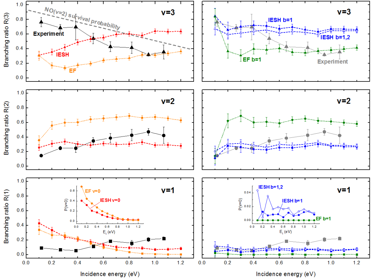
FIG. 3. Branching ratios R(v) for scattering into vibrational states v=1,2,3 . The left panel shows a comparison of experimental data (black symbols, solid line) to the results of IESH (red, dashed) and EF calculations (orange, dotted) when we analyze all trajectories. For comparison, the \text{NO}(v=2) survival probability from Ref. 27 is also shown in the R(3) panel (gray dashed line). The right panel shows the IESH (blue, dashed) and EF (green, dotted) results when the analysis is restricted to trajectories with a single bounce ( b=1 ), compared to the same experimental data. In addition, the right panel shows IESH results for a restriction to trajectories with a single or double bounce ( b=1,2 ; open symbols). The inset diagrams show the calculated absolute probabilities for complete relaxation to v=0 . The error bars on the experimental data indicate statistical uncertainties originating from pulse energy fluctuations of the IR and UV lasers; the error bars on the simulation data represent 2\sigma (95% confidence) statistical uncertainty. Experimentally we find that vibrational relaxation increases with incidence energy at the expense of vibrationally elastic collisions. IESH predicts the wrong dependence on incidence energy, but the restriction to single-bounce trajectories attenuates this trend and yields better agreement with the experimental results. The restriction to single or double-bounce trajectories has a similar but slightly weaker effect. EF predicts much stronger vibrational relaxation from v=3 , and it also exhibits the wrong dependence on incidence energy except at the lowest values. For EF, the selection of single-bounce trajectories also has a strong influence on the E_i dependence. But the most drastic change is that after selection of single-bounce trajectories, relaxation by more than one vibrational quantum, i.e. v=3 \rightarrow 1,0 , is essentially suppressed.
