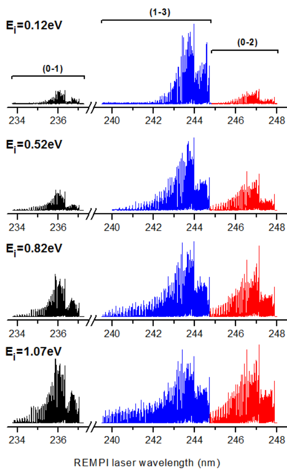
FIG. 1. REMPI spectra, corrected for laser power, detector gain and Franck-Condon factors, recorded at four different incidence energies. The 0-1, 0-2 and 1-3 bands probe the populations of v=1 , 2 and 3 after the scattering process, respectively. For each incidence energy, the three bands are shown on the same scale, illustrating the relative branching. The vertical scales for the different incidence energies were adjusted for optimum visibility. As the incidence energy is increased, the v=1 and v=2 populations grow at the expense of the v=3 population.
