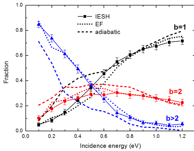
FIG. 5. Fractions of trajectories with b=1 , b=2 or b>2 bounces, as a function of incidence energy, for IESH (solid line with symbols), EF (dotted) and adiabatic (dashed) simulations. We find that the fraction of multi-bounce trajectories drastically increases for lower incidence energies. This behavior is somewhat more pronounced for IESH and EF than for adiabatic simulations, but the general trend is similar for all three models.
