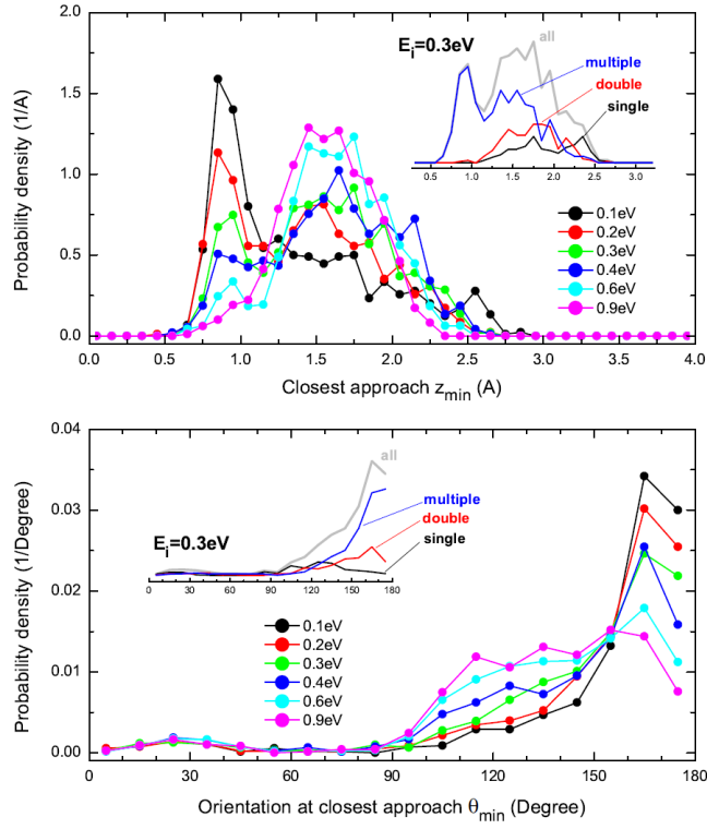
FIG. 11. Distributions for z_{\min} (top) and \theta_{\min} (bottom) at various incidence energies. Top: In addition to a broad feature at 1.2\text{\AA} < z_{\min} < 2.5\text{\AA} , the distributions develop an extra peak, at small values z_{\min} < 1.2\text{\AA} , at smaller incidence energies. The inset diagram presents the distribution for E_i = 0.3\text{eV} along with the distributions for single, double and multiple bounce collisions, clearly showing that the extra peak is exclusively due to multi-bounce collisions. Bottom: The corresponding analysis for \theta_{\min} shows that for low incidence energies, the distributions shift toward 180^\circ (N-down) orientation, but no clear separation is observed as for the z_{\min} distributions. The inset diagram shows that for multi-bounce trajectories, the distributions are narrower and shifted toward 180^\circ as compared to those for single and double-bounce collisions.
