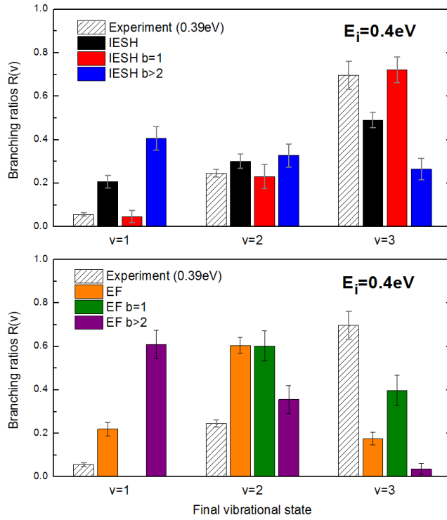
FIG. 10. Branching ratios for vibrational states v=1,2,3 in histogram form. We compare experimental data (hatched bars) to IESH simulations (top) with all trajectories (black), after selection of single-bounce trajectories ( b=1 , red) and after selection of multi-bounce trajectories ( b>2 , blue), and similarly to EF simulations (bottom; all trajectories: orange; b=1 : green; b>2 : purple). The incidence translational energy is E_i=0.39\text{eV} for the experimental data and E_i=0.4\text{eV} for the simulations. For both IESH and EF, the selection of single-bounce trajectories leads to reduced relaxation, whereas the selection of multi-bounce trajectories leads to enhanced relaxation. Only the IESH simulation with a restriction to single-bounce trajectories is in good agreement with the experimental data; however the agreement is not quantitative for all incidence energies.
