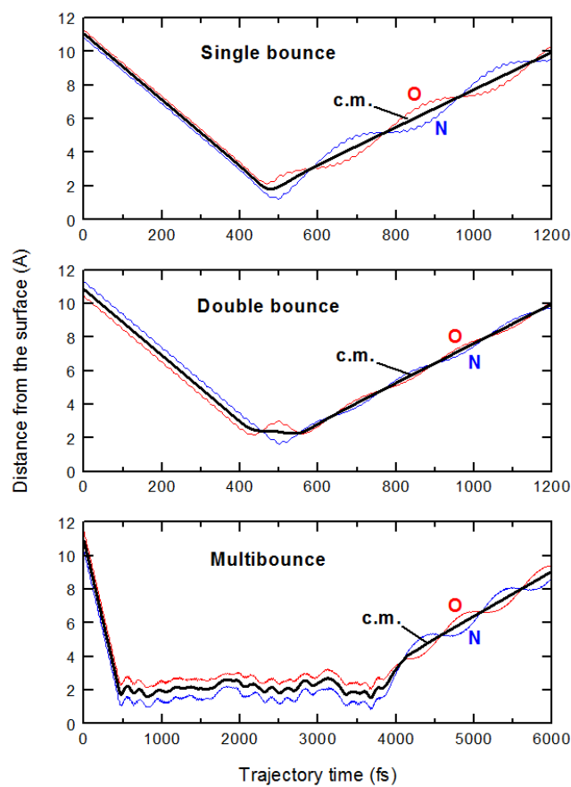
FIG. 4. Typical IESH trajectories for molecule-surface collisions with a single, double, and multiple bounces. The translational incidence energy is 0.6eV in all cases. The blue and red lines show the N and O atom distance from the surface ( z coordinate) as a function of trajectory time. The thick black line shows the corresponding curve for the center of mass of the NO molecule. Looking closely one sees that the single bounce happens for an N-down collision, while the double bounce happens for an O-down collision. For the single bounce, the molecule is still vibrating as it leaves the surface, whereas for the multi-bounce collision it loses most of its vibrational energy. Molecular rotation is excited in all three cases. These observations of course depend on the individual trajectories, but the behavior shown here is quite typical.
