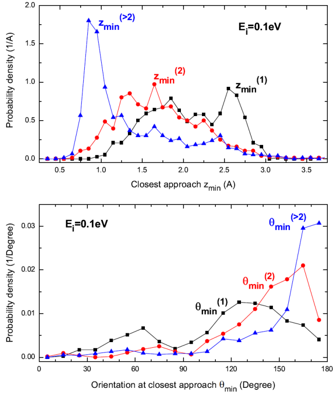
FIG. 8. Distributions for z_{\min}^{(j)} (top) and \theta_{\min}^{(j)} (bottom), i.e. the z_{\min} and \theta_{\min} values assumed during the j -th bounce, for incidence energy E_i=0.1\text{eV} . The values for z_{\min}^{(>2)} and \theta_{\min}^{(>2)} indicate the minimal z_{\min} value assumed during any later-than-second bounce, and the corresponding orientation. The distributions show that the favored geometries, small z_{\min} and \theta_{\min} near 180^\circ , are preferentially assumed during later bounces. Only trajectories with more than two bounces were considered for this analysis.
