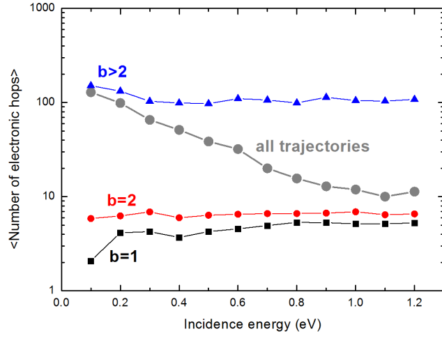
FIG. 6. The average numbers of electronic hops, evaluated for all trajectories (big gray circles) and selectively for single-bounce (black squares), double-bounce (red circles) and multiple-bounce (blue triangles) trajectories. Analyzing all trajectories, we find that the average number of hops drastically increases as the incidence energy is decreased (note the log scale). The detailed analysis shows that the average number of hops is always much higher for multi-bounce than for single and double-bounce trajectories, and that its increase at low E_i is probably due to the increasing fraction of multi-bounce trajectories.
