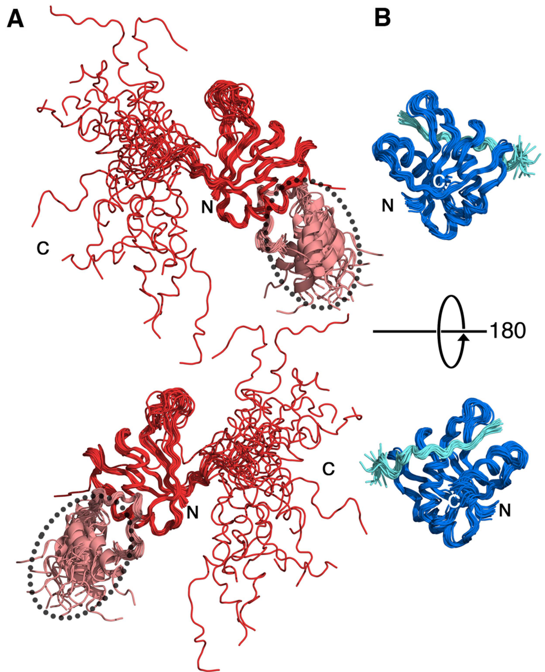
Figure 1. Three-dimensional structures of intermediates during \epsilon RES complex assembly. (A) ^{\text{hC}}\text{Bud13p} - \epsilon Snu17p dimer. 20 lowest-energy structures (backbone atoms only) are shown. Residues 116–131 of Snu17p, which fold into an \alpha -helix in the \epsilon RES trimer 12 , remain flexible in the ^{\text{hC}}\text{Bud13p} - \epsilon Snu17p dimer. In addition, the relative orientation of the C-terminal \alpha -helix of ^{\text{hC}}\text{Bud13p} (marked by a dashed ellipsoid) is flexible. Red, \epsilon Snu17p; pink ^{\text{hC}}\text{Bud13p} . (B) \epsilon Pml1p- \epsilon Snu17p dimer. Shown are the backbones of the 20 lowest-energy structures of the NMR ensemble. Blue, \epsilon Snu17p; cyan \epsilon Pml1p.
