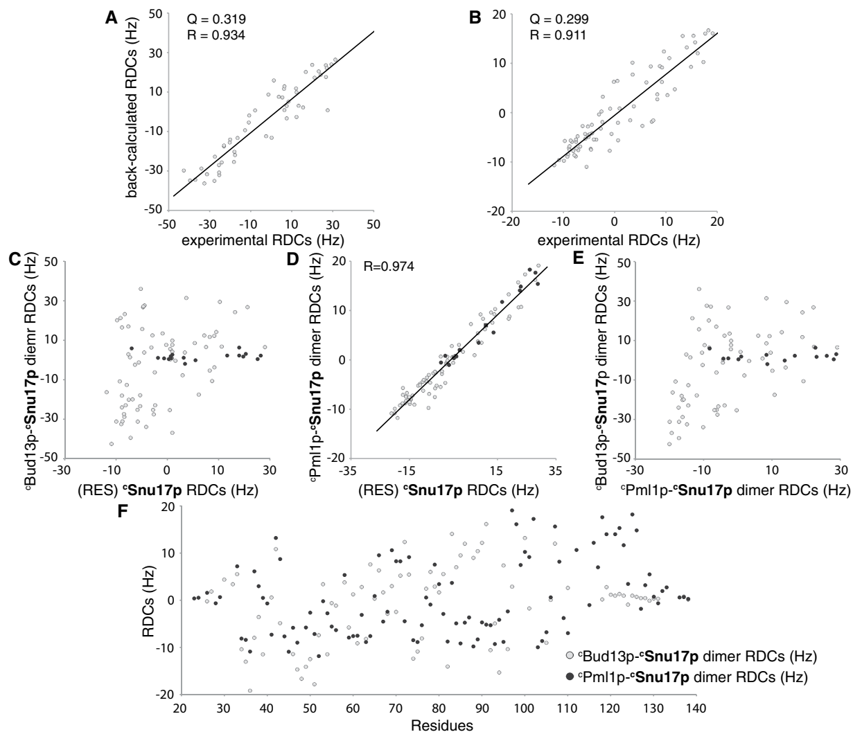
Figure 3. Analysis of HN RDCs observed in ^15\text{Snu17p} when part of the ^15\text{Pml1p} - ^15\text{Snu17p} dimer, the ^{13}\text{Bud13p} - ^15\text{Snu17p} dimer and ^15\text{RES} . (A,B) Comparison of experimental RDCs with values back-calculated from the 3D structure of the ^15\text{Pml1p} - ^15\text{Snu17p} dimer (A) and the ^{13}\text{Bud13p} - ^15\text{Snu17p} dimer (B). (C,D) Comparison of RDCs observed in ^15\text{Snu17p} in ^15\text{RES} with RDCs observed in ^15\text{Snu17p} when part of the ^{13}\text{Bud13p} - ^15\text{Snu17p} dimer (C) or the ^15\text{Pml1p} - ^15\text{Snu17p} dimer (D). Black dots indicate disordered C-terminal residues in the ^{13}\text{Bud13p} - ^15\text{Snu17p} dimer. (E) Comparison of RDCs observed in ^15\text{Snu17p} in complex with ^15\text{Snu17p} and in complex with ^{13}\text{Bud13p} . Black dots indicated disordered C-terminal residues in ^{13}\text{Bud13p} - ^15\text{Snu17p} dimer. (F) Residue-specific comparison of RDCs observed in dimeric complexes of ^15\text{Snu17p} with ^15\text{Pml1p} and with ^{13}\text{Bud13p} . In (F), RDC values of the ^{13}\text{Bud13p} - ^15\text{Snu17p} dimer were normalized to the magnitude of the alignment tensor of the ^15\text{Pml1p} - ^15\text{Snu17p} dimer.
