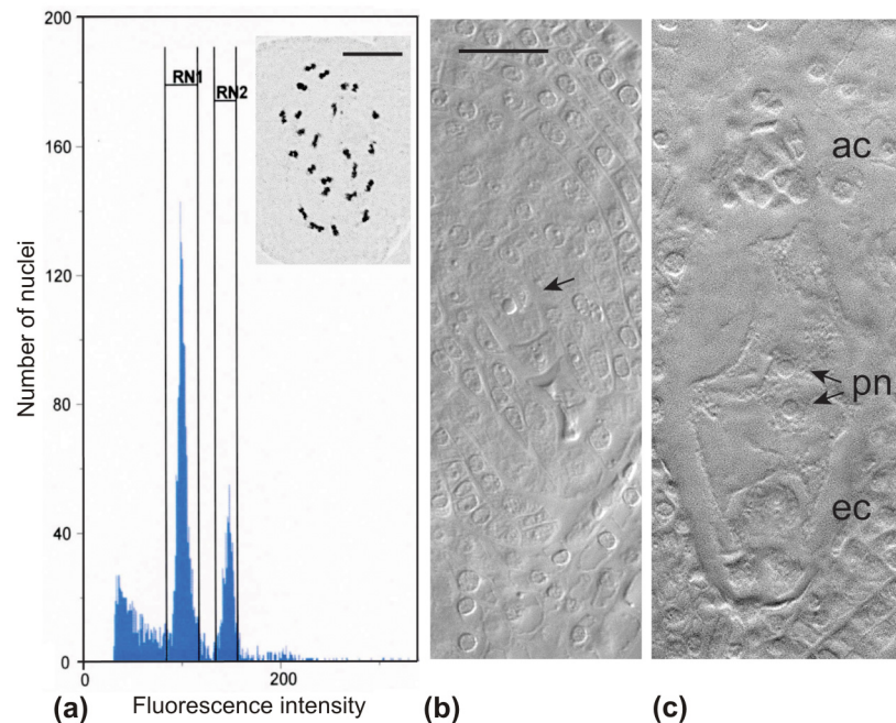
Fig 6. Ovule and seed development in Centotheca lappacea . (a) Single seed flow cytometry histogram of 3000 nuclei from genotype HJ3-01 showing the characteristic 2:3 ratio (relative peak positions of ~100 and ~150 on the x-axis) between the embryo (RN1, diploid) and endosperm (RN2, triploid) ploidy levels corresponding to a seed formed via a sexual reproductive pathway. The mitotic metaphase cell showing 2n = 2x = 24 chromosomes corresponds to a diploid maternal plant from HJ3 population, and further supports diploidy on seed embryos. (b) End of megasporogenesis showing four meiotic products, the two toward the micropyle aborted. The arrows indicate the functional megaspore (from genotype BJ2-16). (c) Mature female gametophyte at the time of anthesis (from genotype BO1-2). After development of the characteristic Polygonum -type embryo sac carrying three antipodal cells, extra mitotic divisions produce a mass of antipodal cells (ac) at the chalazal embryo sac pole. Further abbreviations: ec (egg cell), pn (polar nuclei). Scale bars represent 20 \mu m.
