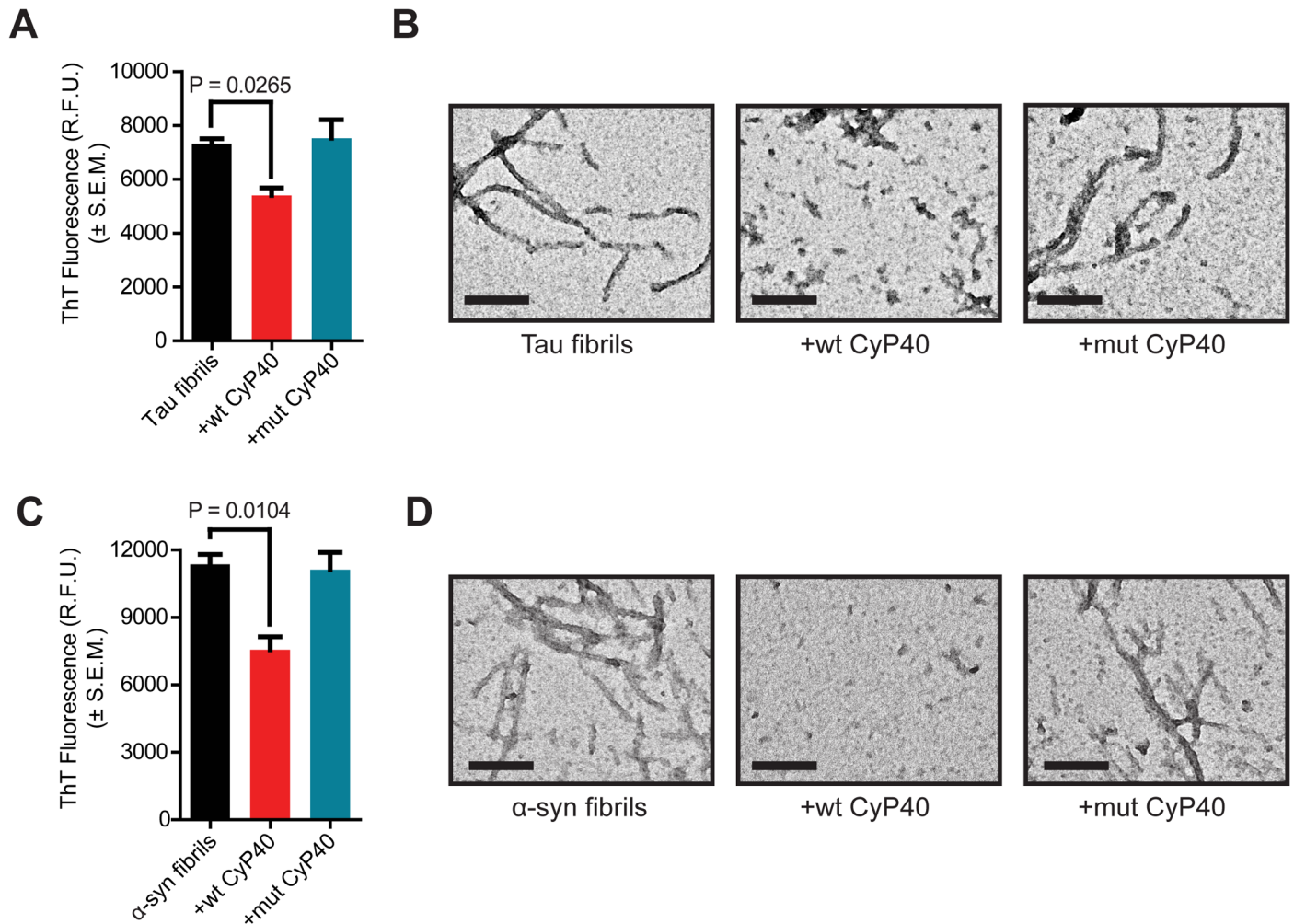
Fig 7. Cyclophilin 40 (CyP40)-mediated disaggregation assay of wild-type (wt) and peptidyl-prolyl isomerase (PPIase) null mutant (mut) CyP40. (A) Thioflavin T (ThT) fluorescence of tau ± wt CyP40 or mut CyP40 (unpaired t test, n = 3 for each condition). (B) Representative transmission electron microscopy (TEM) images of (A) (scale bar 200 nm). (C) ThT fluorescence of A53T α-synuclein (α-syn) ± wt CyP40 or mut CyP40 (unpaired t test, n = 3 for each condition). (D) Representative TEM images of (C) (scale bar 200 nm). The numerical data used in panels 7A and 7C can be found in S1 Data . RFU, relative fluorescence unit; SEM, standard error of the mean.
