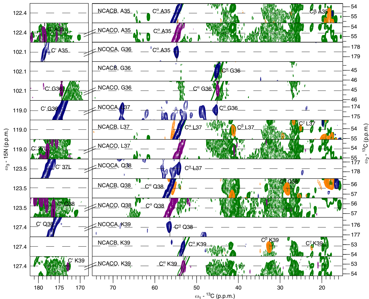
Figure 2 | Sequence-specific resonance assignment of membrane-embedded mTSPO (bound to DAA1106). Strip plots of 3D NCACB (diagonal peak—blue, cross peak—orange), 3D NCOCA (cross peak—blue) and NCACO (cross peak—purple) used for sequence-specific resonance assignments. Corresponding regions from the 2D proton-driven spin diffusion (green) are superimposed for comparison.
