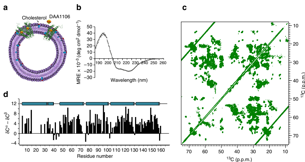
Figure 1 | High-resolution solid-state NMR of mammalian TSPO in a lipid bilayer. (a) Schematic representation of mammalian TSPO embedded into liposomes. Cholesterol is marked in red and cyan, the TSPO-ligand DAA1106 in orange/yellow. (b) CD spectrum of the membrane-embedded mTSPO/DAA1106 complex. (c) High-resolution 13 C– 13 C proton-driven spin diffusion spectrum of mTSPO bound to DAA1106. (d) Secondary structure analysis of liposome-embedded mTSPO in complex with DAA1106. Positive \delta C^{\alpha} - \delta C^{\beta} values are indicative of \alpha -helix and identify five transmembrane helices and a short cytosolic helix following transmembrane helix I.
