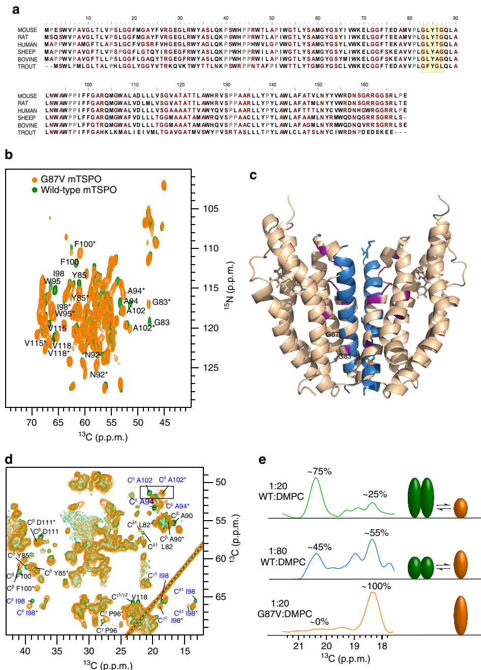
Figure 3 | Mammalian TSPO populates a dynamic monomer/dimer equilibrium in the membrane. (a) Conservation of the amino acid sequence of mammalian TSPO. The GxxxG motif in transmembrane helix III is highlighted in yellow. (b) Superposition of nitrogen-carbon correlation spectra of wild-type mTSPO (green) and its G87V mutant (orange) both in complex with DAA1106. Residues, which show two cross-peaks, are labelled. Peaks corresponding to the mTSPO monomer are marked by stars. (c) Model of the mTSPO dimer with an interhelical arrangement as observed in glycoporphin A (shown in blue). Residues that show two cross-peaks in b are highlighted in purple. (d) Superposition of carbon-carbon correlation spectra of wild-type mTSPO/DAA1106 (green) and its G87V variant (orange). The C α /C β peaks of A102, which were used for monomer/dimer quantification, are highlighted. Residues with two conformations (two peaks in proton-driven spin diffusion /NCA/NCACB) are marked in blue. Residues with shifted side-chain resonances are labelled in black. (e) One-dimensional traces at the C β resonance of A102 in wild-type mTSPO at protein-to-DMPC molar ratios of 1:20 (top) and 1:80 (middle). In case of the G87V-mTSPO, only the monomer peak of A102 was observed (bottom).
