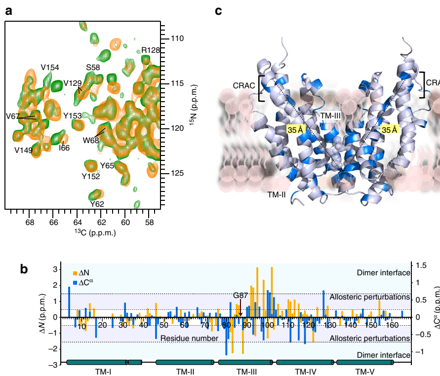
Figure 4 | TSPO dimerization is coupled to long-range changes in the tertiary structure of TSPO. (a) Residues up to 35 Å away from mTSPO's 83 GxxxG 87 oligomerization motif experience changes in their chemical environment upon protein monomerization. NCA spectra of wild-type TSPO/DAA1106 and its G87V mutant are shown in green and orange, respectively. Perturbed residues include Y153 and V154 in TSPO's cholesterol-binding motif. (b) Residue-specific chemical shift differences between the dimeric and monomeric form of mTSPO (both in complex with DAA1106). Chemical shift perturbations \Delta N > 1.5 p.p.m. and \Delta C^{\alpha} > 0.75 p.p.m. were observed near the dimer interface. Additional chemical shift perturbations ( 0.5 < \Delta N < 1.5 p.p.m., 0.25 < \Delta C^{\alpha} < 0.75 p.p.m.) report on allosteric changes. (c) Residues with 13 C chemical shift perturbations > 0.25 p.p.m. in b were mapped in blue colour onto the dimer model of mTSPO. G83 and G87, which form the GxxxG oligomerization motif in TM-III, are represented by spheres.
