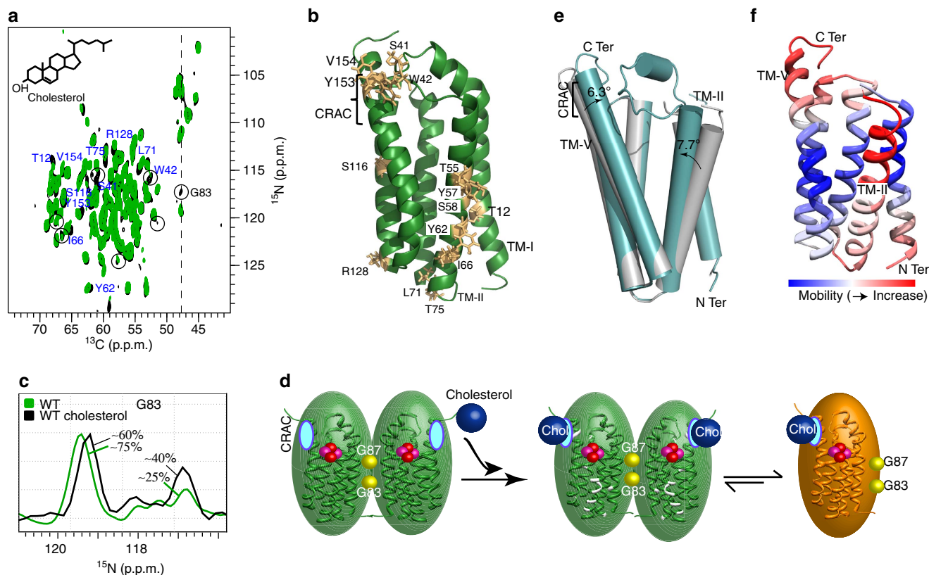
Figure 5 | An allosteric signal pathway that connects cholesterol binding to membrane protein tertiary and quaternary structure. (a) Comparison of solid-state NMR spectra of mTSPO (bound to DAA1106) in the absence (green) and presence (black) of a tenfold excess of cholesterol. Residues that undergo chemical shift changes are labelled. Circled cross-peaks increase in intensity. (b) Residues affected in a are highlighted in gold on the 3D structure of mTSPO (PDB id: 2MGY). The cholesterol-binding motif (CRAC) in TM-V is indicated. (c) Quantification of the dimer/monomer equilibrium in the absence (green) and presence (black) of cholesterol. Spectral traces at the C^\alpha chemical shift of G83 (dashed line in a) are shown. (d) Schematic representation illustrating the connection between cholesterol binding, allosteric changes in tertiary structure (marked in white) and TSPO dimer dissociation. The CRAC motif before binding of cholesterol is shown in cyan. DAA1106 is shown in a sphere representation (pink/red). In the mTSPO monomer (gold), the ^{83}\text{GxxxG}^{87} motif in TM-III is available for interaction with other proteins of the outer mitochondrial membrane. (e) Crystal structures of bacterial proteins (PDB id: 4UC2 (green) and 4UC3 (grey)), which are homologous to mammalian TSPO, highlight the ability of transmembrane helices TM-V and TM-II to undergo changes in transmembrane orientation. (f) Mobility of different regions in the TSPO fold as predicted by Gaussian network analysis. Gaussian network analysis was performed for PDB id 4UC3. The least stable transmembrane parts of the TSPO fold are the CRAC motif in TM-V and the transmembrane helix TM-II.
