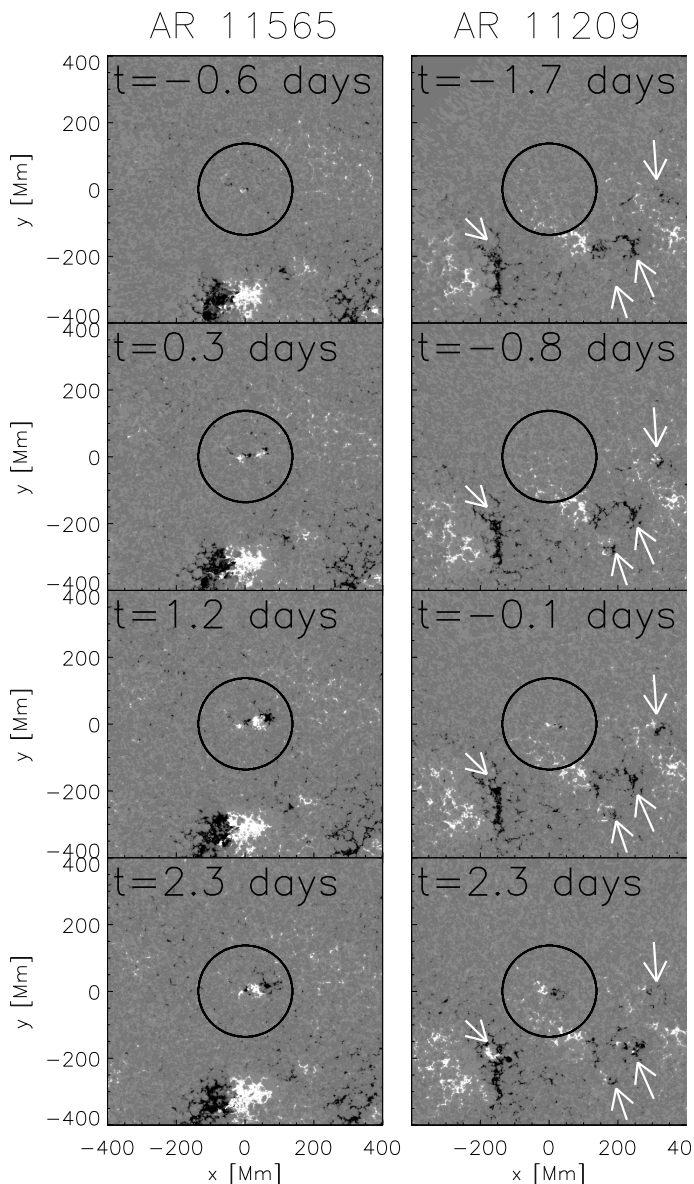
Fig. 8. Evolution of the line-of-sight magnetic field of two emerging active regions, AR 11565 (left column) and AR 11209 (right column). AR 11565 shows a double emergence and AR 11209 is a smaller active region with many surrounding small emergences pointed to by the arrows. The black circle indicates a radius of 10^\circ from the centre of the emerging active region. The greyscale is saturated at \pm 200 G.
