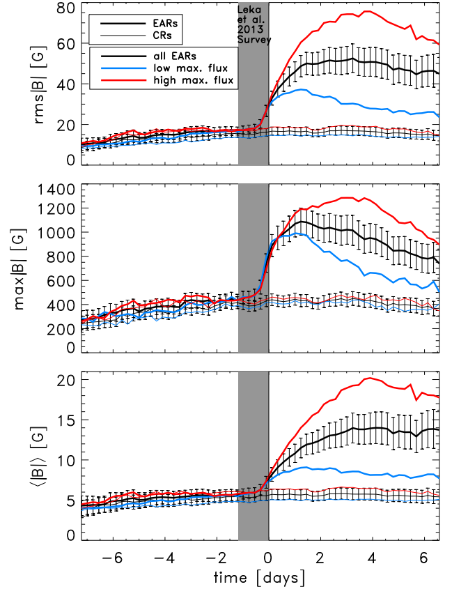
Fig. 7. Mean (bottom panel), maximum (middle panel), and rms (top panel) of the absolute line-of-sight magnetic field in the central 10^\circ radius averaged over all emerging active regions (thick black) at each time interval. The blue curve shows the values for only those active regions that reach a maximum flux that is lower than the median maximum flux value, and the red curve shows the values for the emerging active regions that reach a higher value. The corresponding values for the control regions are shown by the thin curves. The shaded grey area indicates the time span covered by the previous LBB survey. The uncertainties are the rms of the quantity. For example, in the top panel, \sigma_{B_{\text{rms}}} = \sqrt{\sum B_{\text{rms}}^2 / N} , where N is the number of active regions at time interval, TI.
