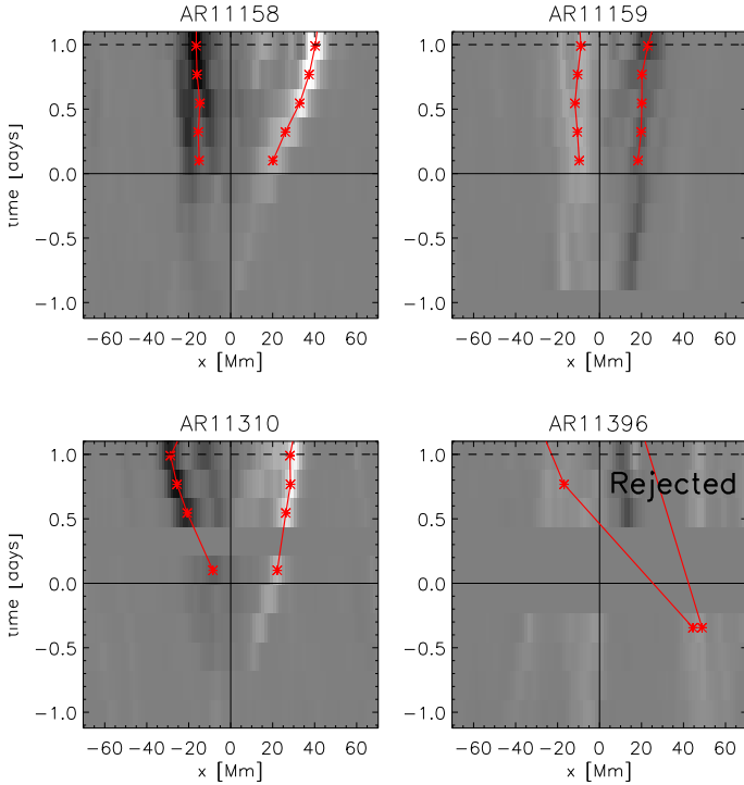
Fig. 10. Examples of the temporally averaged line-of-sight magnetic field averaged over the central 15 Mm in the y direction for selected emerging active regions. The greyscale is saturated at \pm 500 G. The red crosses show the centre of the fitted Gaussian to the leading (positive x direction) and trailing (negative x direction) polarities.
