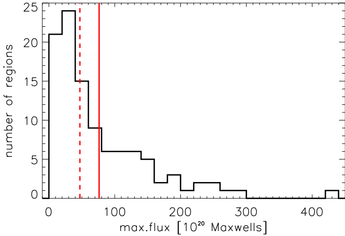
Fig. 2. Number of EARs as a function of maximum total unsigned flux. The solid red vertical line indicates the mean and the dashed line indicates the median value. Active regions indicated with asterisks in Table A.1 are those with values greater than the median.
