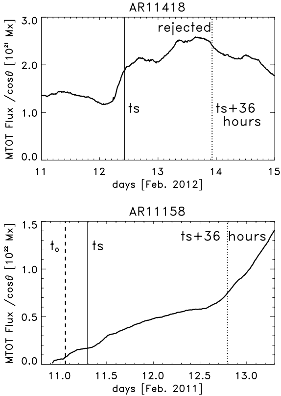
Fig. 1. Corrected MTOT flux as a function of time for two example emerging active region candidates. The solid line represents the time, t_s , when NOAA first recorded a numbered sunspot region. The top panel shows an example of an emerging sunspot group, AR 11418, which we rejected from our survey. While an increase of new flux is apparent near the time t_s , it is obvious that considerable flux already exists within the SHARP boundary. The bottom panel shows an example, AR 11158, which we included in the survey. The thick dashed line indicates the emergence time t_0 when the flux was 10% of its peak value within the interval bounded by the solid and dotted lines, t_s and t_s + 36 h, respectively.
