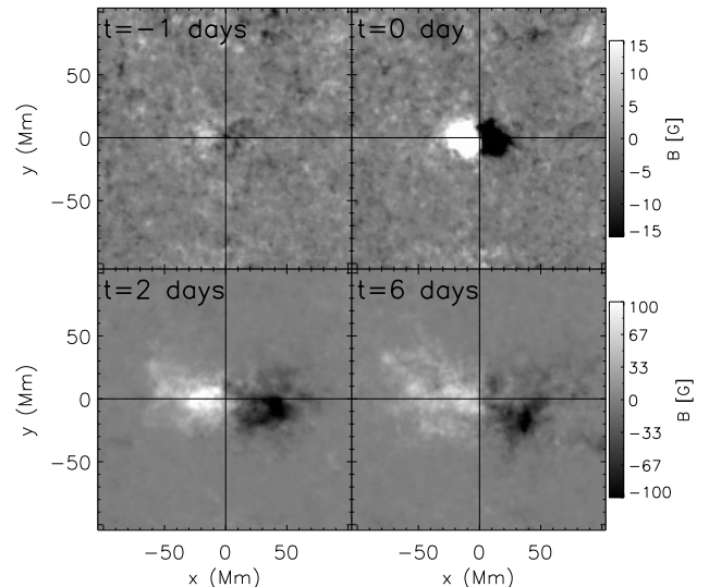
Fig. 9. Average line-of-sight magnetic field maps for all EARs at selected time intervals. The southern hemisphere active regions have had their polarity reversed and have been flipped in the y direction to account for Hale’s law.
