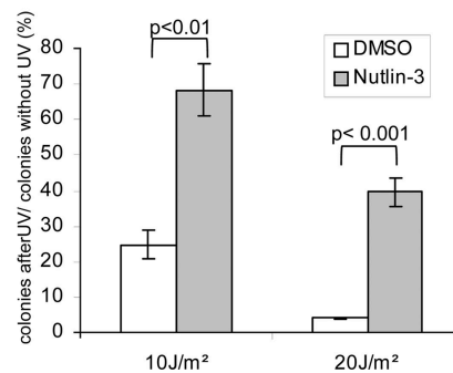
Figure 4. Nutlin-3 enhances long-term survival upon UV irradiation. (A) U2OS cells were treated with 8 \mu M Nutlin-3 or the solvent DMSO. After 24 h, they were UV irradiated. The cell cycle profile was determined by FACS analysis 24 h after irradiation. The percentage of cells in the sub-G1 fraction (M1) is indicated (top). For the bottom panel, the cells were first treated the same way. After harvesting, they were incubated with annexin V-FITC, counterstained with propidium iodide, and analyzed by flow cytometry. Percentages of cells in each quadrant were determined. (B) U2OS cells were seeded in triplicate at 500 cells per 3.5-cm dish. Thereafter, they were treated with 8 \mu M Nutlin-3 or DMSO. After 24 h, the cells were UV irradiated or not irradiated followed by further incubation with Nutlin-3 or DMSO for another period of 24 h. Thereafter, the drug was removed, and the medium was replaced. After 7 (no UV; 10 J/m 2 ) or 10 d (20 J/m 2 ), emerging colonies were stained with crystal violet. The results represent the percentage of surviving colonies and are shown as the means from three independent experiments with their corresponding SEM (error bars).
