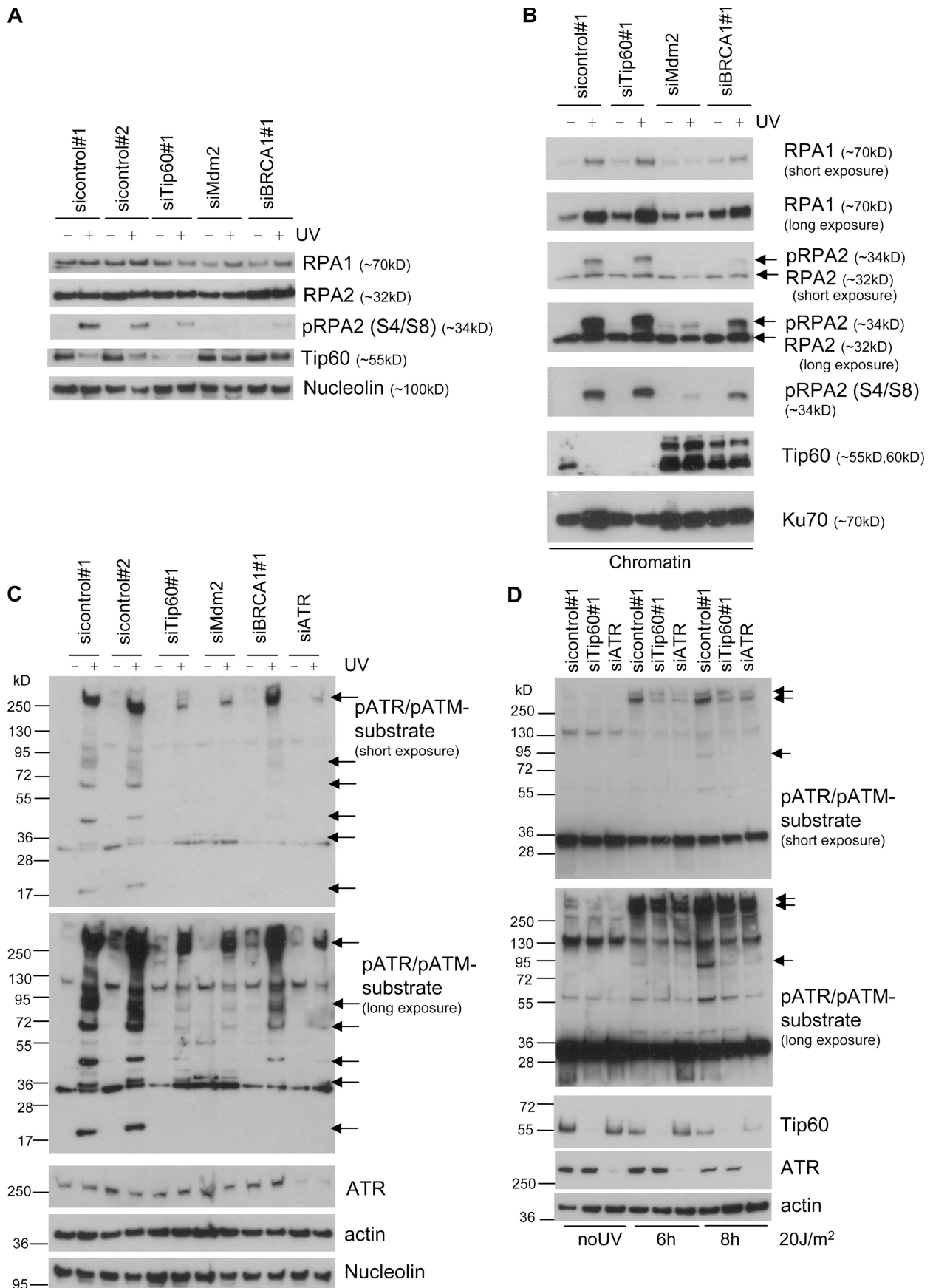
Figure 8. Knockdown of Mdm2 or BRCA1 but not Tip60 impairs RPA2 phosphorylation and RPA1/RPA2 recruitment to chromatin, whereas all three siRNA species diminish the phosphorylation of ATR substrates. (A) U2OS cells were transfected with 30 nM siRNA and UV irradiated (20 J/m 2 ) followed by
