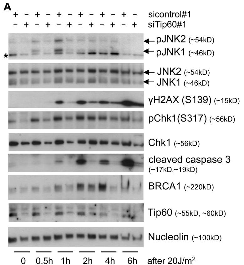
Figure 2. Impairment of the response to UV irradiation by Tip60 knockdown is independent of p53. (A) Saos-2 cells were transfected with 30 nM siRNA (siTip60#1 or sicontrol#1). 48 h later, cells were exposed to 20 J/m 2 UV and harvested after the indicated time points for Western blotting. The asterisk indicates a nonspecific band. (B) Saos-2 cells were transfected with 30 nM of the indicated siRNAs and UV irradiated (20 J/m 2 ) 48 h later. 48 h after UV irradiation, cells were harvested for FACS analysis, and the percentage of sub-G1 cells was determined. The results shown represent the mean percentages of sub-G1 cells from four independent experiments with their corresponding SD (error bars).
