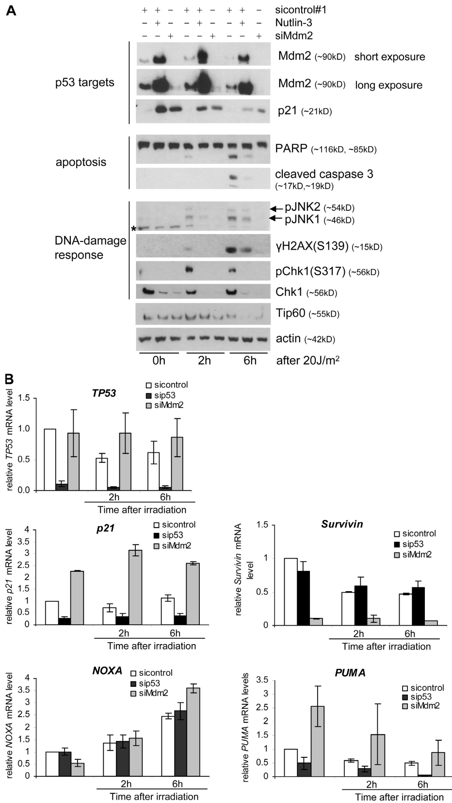
Figure 3. Pharmacological as well as siRNA-mediated preactivation of p53 inhibits the UV response. (A) U2OS cells were transfected with 30 nM siRNA (sicontrol#1 or siMdm2). After 24 h, cells were treated with 8 \mu M Nutlin-3 or the solvent DMSO. After an additional incubation for 24 h, the cells were UV irradiated (20 J/m 2 ) and harvested 0, 2, and 6 h after irradiation for Western blotting. The asterisk indicates a nonspecific band. (B) Quantitative real-time PCR analysis of TP53 , p21 , Survivin , NOXA , and PUMA mRNA in U2OS cells was performed to determine the corresponding relative mRNA levels after transfection with 30 nM of the indicated siRNAs 0, 2, and 6 h after UV irradiation (20 J/m 2 ). Glyceraldehyde 3-phosphate dehydrogenase mRNA was used as an internal control. Error bars represent SD.
