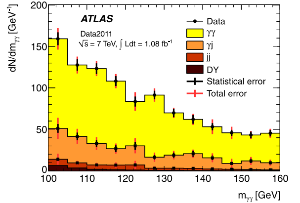
Fig. 2. Diphoton, photon-jet, dijet and Drell–Yan contributions to the diphoton candidate invariant mass distribution, as obtained from a data-driven method. The various components are stacked on top of each other. The error bars correspond to the uncertainties on each component separately.
