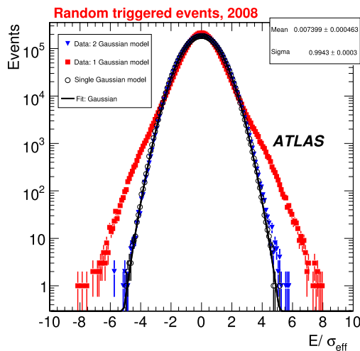
Fig. 11 Significance level of the cell energy as compared to noise ( E/\text{Gaussian } \sigma ) using the single and the double Gaussian descriptions of noise in random triggered events
