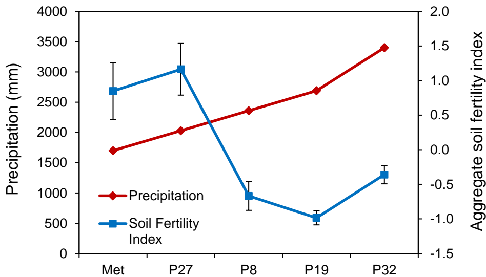
Figure S2 above - the factor 1 and 2 scores of the five variables ( \delta^{15}\text{N} enrichment factor, effective cation exchange capacity (ECEC), exchangeable soil aluminum, soil C:N ratio and % clay content) included in the principal component analysis for determining an aggregate soil fertility index for each site; below - the five lowland forest sites along orthogonal gradients of annual precipitation and soil fertility in the Panama Canal watershed, central Panama. Standard error bars of soil fertility indices are determined from four replicate plots per site.
