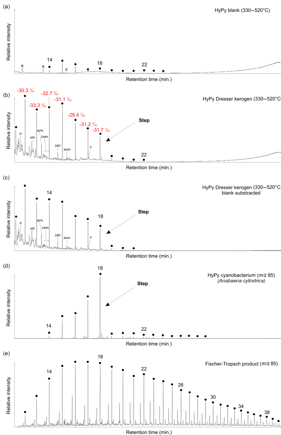
Figure 3. Total ion currents (a–c; on the same scale) and ion chromatograms selective for alkanes (d–e; m/z 85). (a) High-temperature HyPy (330–520 °C) product of analytical blank (combusted sea sand) obtained prior to HyPy of the Dresser kerogen. n -Alkanes in the range of n -C 14 to n -C 24 (maxima at n -C 15 ) represent HyPy background contamination. (b) High-temperature HyPy (330–520 °C) product of the Dresser kerogen. Note the sharp decrease in abundance of n -alkanes beyond n -C 18 (see arrows). \delta^{13}\text{C} values of n -C 12 to n -C 28 show a high similarity to the \delta^{13}\text{C}_{\text{TOC}} value ( -32.8 \pm 0.3\text{‰} ), further confirming syngeneity. (c) Blank subtraction (b minus a) showing that contaminants have no major impact on the n -alkane pattern yielded during the high-temperature HyPy step of the Dresser kerogen (b). (d) HyPy products of cell material of the heterocystous cyanobacterium Anabaena cylindrica . Note the sharp decrease in abundance of n -alkanes beyond n -C 18 (see arrows), similar to the n -alkane distribution of the Dresser kerogen (b). (e) Products of experimental Fischer–Tropsch-type synthesis under hydrothermal conditions; abiogenic n -alkanes show a unimodal distribution that is distinctly different from the Dresser kerogen. Black dots: n -alkanes (numbers refer to carbon chain lengths); N: naphthalene; MN: methylnaphthalenes; BiPh: 1,1'-biphenyl; DMN: dimethylnaphthalenes; DBF: dibenzofuran; MAN: methylacenaphthene; P: phenanthrene; crosses: siloxanes (GC column or septum bleeding).
