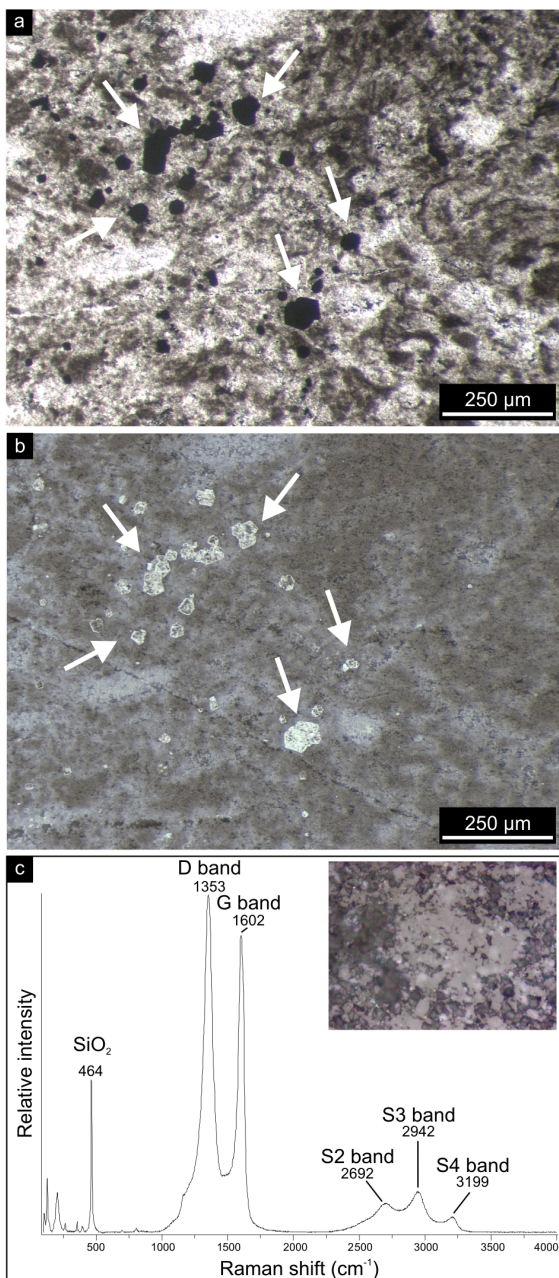
Figure 2. Petrographic observations on the hydrothermal chert vein. (a, b) Thin section photographs ( a transmitted light; b reflected light) showing kerogen (brownish colours) and pyrite (arrows, black colours in a , bright colours in b ) embedded within a fine-grained chert matrix. Note that the pyrite crystals (arrows) are excellently preserved and show no evidence of oxidation. (c) Representative Raman spectrum of kerogen (D band at 1353\text{ cm}^{-1} and G band at 1602\text{ cm}^{-1} ) present in the hydrothermal chert vein. Note the wide D and G bands ( 82 and 55\text{ cm}^{-1} width, respectively), pointing to thermally mature and structurally disordered kerogen, and the absence of an S1 band (at 2450\text{ cm}^{-1} ), consistent with prehnite–pumpellyite to lower greenschist metamorphism and a temperature of ca. 300\text{ }^{\circ}\text{C} (cf. Yui et al., 1996; Delarue et al., 2016).
