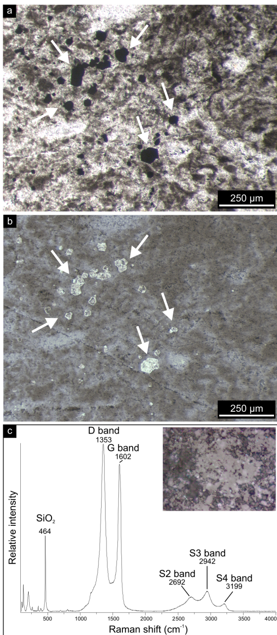
Figure 2. Petrographic observations on the hydrothermal chert vein. (a, b) Thin section photographs (a transmitted light; b reflected light) showing kerogen (brownish colours) and pyrite (arrows, black colours in a, bright colours in b) embedded within a fine-grained chert matrix. Note that the pyrite crystals (arrows) are excellently preserved and show no evidence of oxidation. (c) Representative Raman spectrum of kerogen (D band at 1353\text{ cm}^{-1} and G band at 1602\text{ cm}^{-1} ) present in the hydrothermal chert vein. Note the wide D and G bands ( 82 and 55\text{ cm}^{-1} width, respectively), pointing to thermally mature and structurally disordered kerogen, and the absence of an S1 band (at 2450\text{ cm}^{-1} ), consistent with prehnite–pumpellyite to lower greenschist metamorphism and a temperature of ca. 300\text{ }^{\circ}\text{C} (cf. Yui et al., 1996; Delarue et al., 2016).
