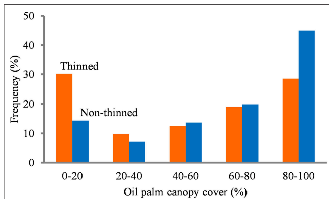
FIGURE 3 | Distribution of oil palm canopy cover in thinned and non-thinned plots where trees were planted ( N_{\text{thinned}} = 24,870 pixels and N_{\text{non-thinned}} = 307 pixels, in 48 plots).
