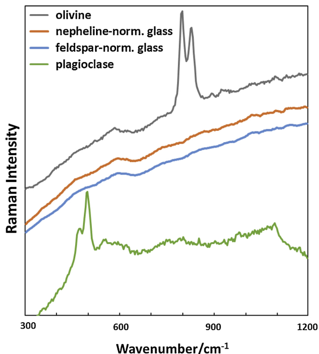
Fig. 6. Raman spectra of olivine, nepheline-normative glass from the coarse-grained lithology in the thick section A, and plagioclase from the fine-grained lithology in the thin section. Olivine is identified by two characteristic peaks at \sim 820 \text{ cm}^{-1} and \sim 840 \text{ cm}^{-1} and plagioclase by two peaks at \sim 481 \text{ cm}^{-1} and \sim 510 \text{ cm}^{-1} . The feldspar- and the nepheline-normative glasses are featureless with increasing intensity due to increase of fluorescence. The spectra are not corrected for the background emission.
