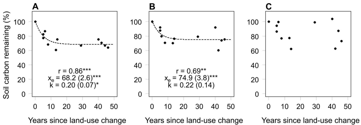
Figure 2. Soil carbon remaining after land-use change at (A) 0–0.15-m, (B) 0.15–0.3-m, and (C) 0.3–0.6-m depth. Soil carbon remaining is expressed as the proportion of soil carbon in rubber plantations relative to the secondary forest. The dashed lines represent fitted mono-exponential models (see Equation 2). r = Pearson’s correlation coefficient between observed and fitted values; k = decay rate (year -1 ) and X e = equilibrium ratio (%), and values in brackets are SE. Pearson’s r and parameter estimates are significant at * P ≤ 0.05, ** P ≤ 0.01, and *** P ≤ 0.001. doi:10.1371/journal.pone.0069357.g002
