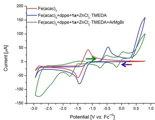
Scheme 4. CVs recorded at 100\text{ mV s}^{-1} with n\text{Bu}_4\text{NPF}_6 (0.1 M in THF), concentrations of substrates 5 mM ( \text{ArMgBr} 20 mM). (a) DCIB. (b) Ligand effect. (c) Additive and Grignard agent.
