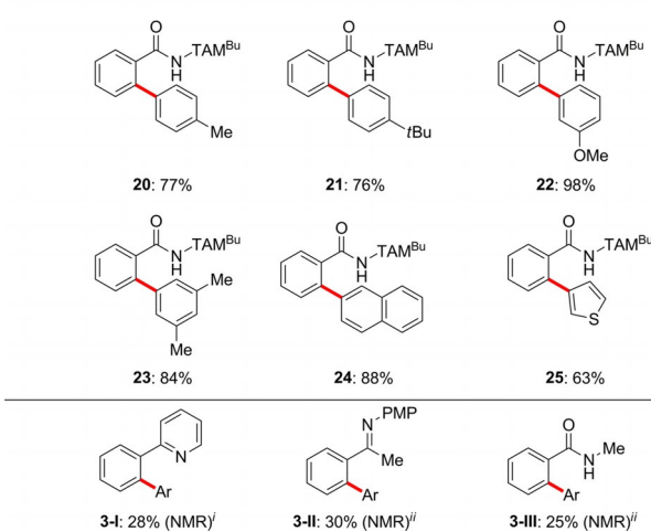
Scheme 1. Robustness of the electrochemical C–H arylation of amides 1 . (a) The iron-electrocatalysis enabled direct arylations of various arenes, ferrocenes and heteroarenes with excellent levels of mono-, chemo-, and site-selectivity, Ar = 4-MeOC 6 H 4 . (b) Various aryl motifs could be introduced by the electrooxidative C–H activation. (i) 1,10-phenanthroline as ligand. (ii) 4,4'-di- tert -butyl-2,2'-bi-pyridyl (dtbpy) as ligand.
