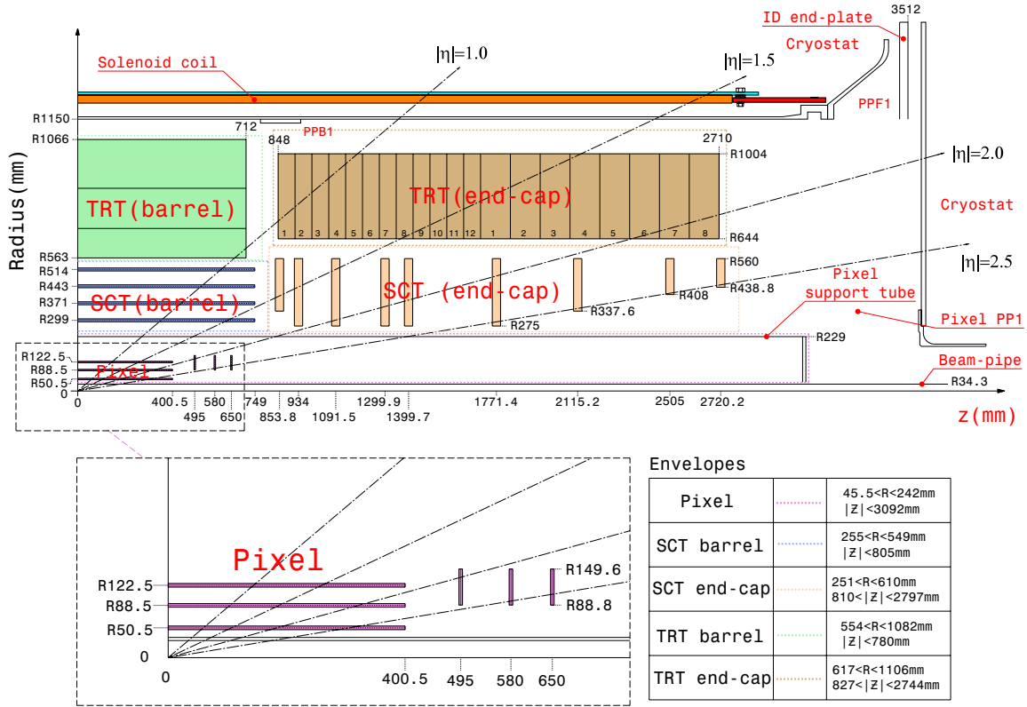
Figure 1. View of a quadrant of the ID [5] showing each of the major detector elements with their active dimensions and envelopes. The lower part shows a zoomed-in view of the pixel detector region.
