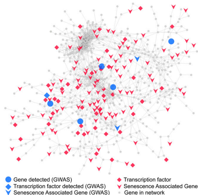
Figure 3. A Major Coexpression Subnetwork Underlying Stay-Green.
