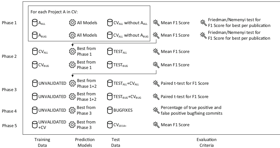
Fig. 7 Overview of the experiment methodology. The training and evaluation in all phases is conducted with all issues and with only bug issues
