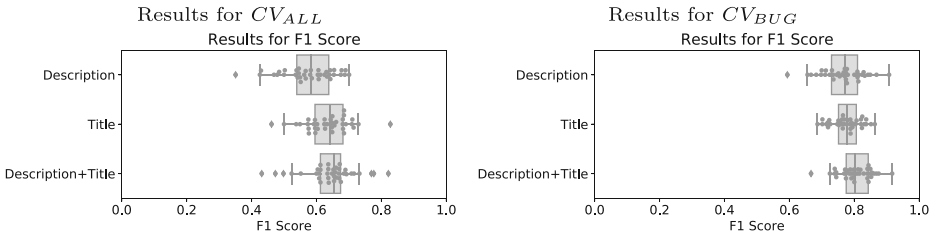
Fig. 10 Results for the different classifiers for title and description in comparison to their combination to gain insights into the Herbold2020-FTA model
