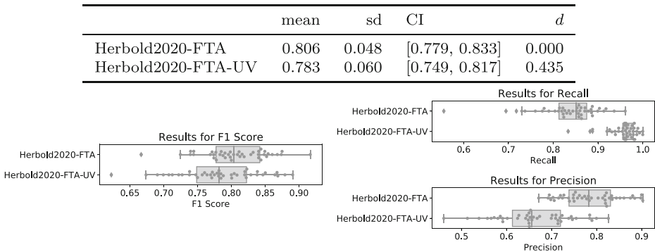
Fig. 14 Comparison of the results from Phase 1 and Phase 2 with training with the UNVALIDATED data and testing with CV_{BUG} and TEST_{BUG}
