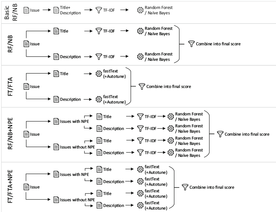
Fig. 5 Summary of our approach
