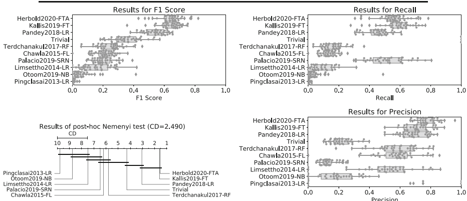
Fig. 8 Results of leave-one-project-out cross validation with the CV_{ALL} data. The bold-faced approaches where the best for a publication and are used in the statistical analysis
