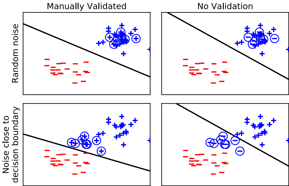
Fig. 6 Example for the possible effect of mislabels in the training data on prediction models. The color indicates the correct labels, i.e., red for bugs and blue for other issues. The marker indicates the label in the training data, - for bugs, + for other issues. Circled instances are manually corrected on the left side and mislabels on the right side. The line indicates the decision boundary of the classifier. Everything below the line is predicted as a bug, everything above the line is predicted as not a bug
