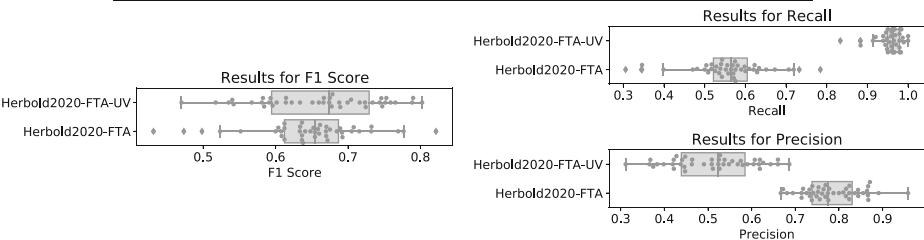
Fig. 13 Comparison of the results from Phase 1 and Phase 2 with training with the UNVALIDATED data and testing with CV_{ALL} and TEST_{ALL}
