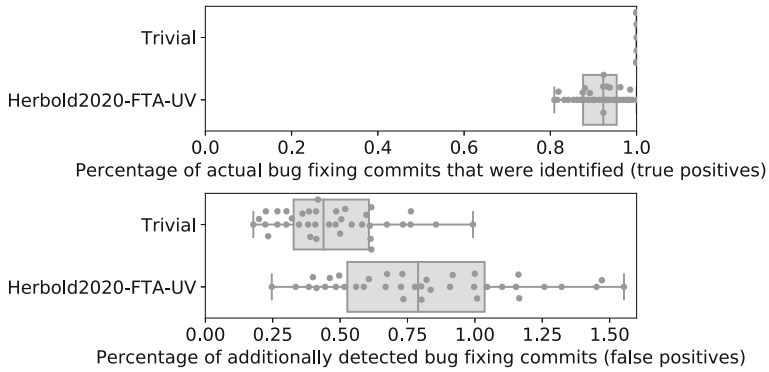
Fig. 15 Impact on using Herbold2020-FTA-UV for the labeling of bugfixing commits
