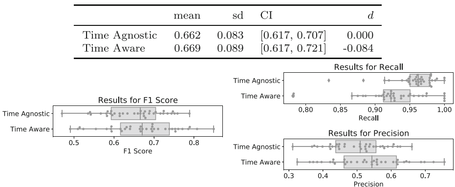
Fig. 16 Evaluation in a realistic time aware setting in comparison to the time agnostic results from Phase 3. The results from Phase 3 are restricted to the projects we evaluate in Phase 5, i.e., the projects from CV without commons-digester
