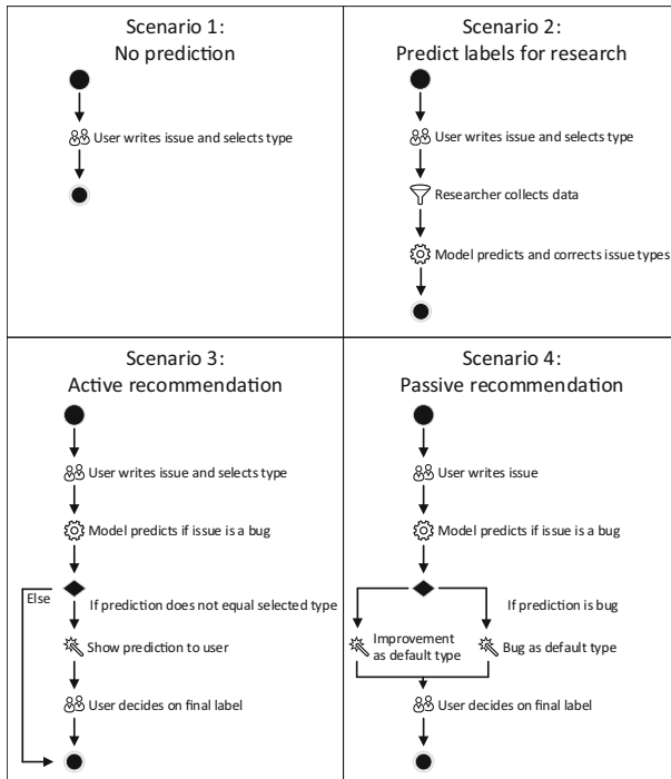
Fig. 2 Overview of the scenarios how prediction systems for bug issues can be used
