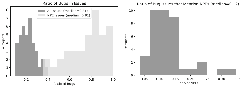
Fig. 4 Data on the usage of the terms NullPointerException , NPE , and NullPointerException in issues based on 30,922 issues from the CV data (see Section 6.1)
