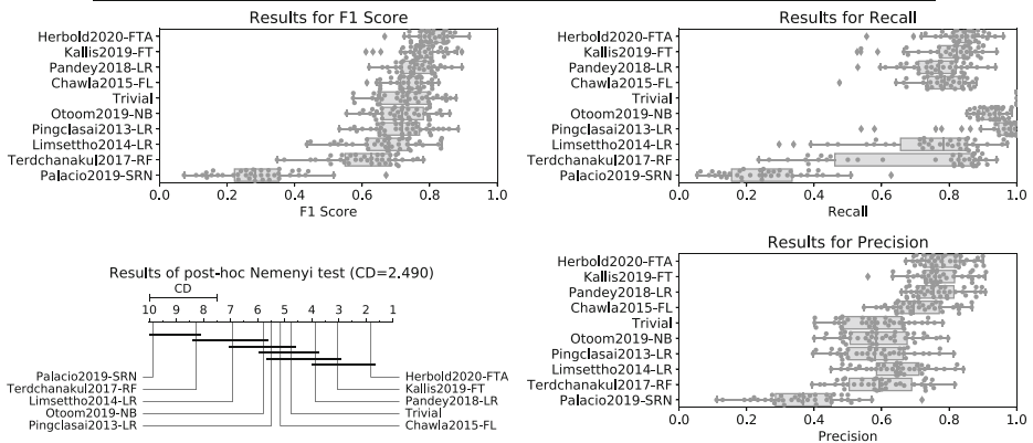
Fig. 9 Results of leave-one-project-out cross validation with the CV_{BUG} data. The bold-faced approaches where the best for a publication and are used in the statistical analysis
