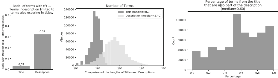
Fig. 3 Visualization of the structural differences of issue titles and descriptions based on the 607,636 Jira Issues from the UNVALIDATED data (see Section 6.1)
