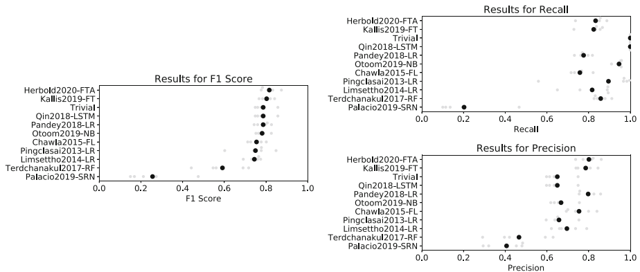
Fig. 12 Results of training with the CV_{BUG} and testing with the TEST_{BUG} data
