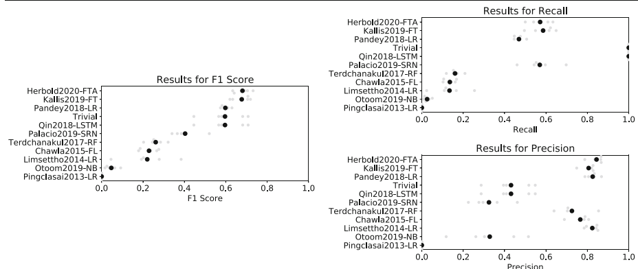
Fig. 11 Results of training with the CV_{ALL} and testing with the TEST_{ALL} data
