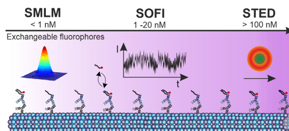
Figure 3. Comparison of super-resolution imaging methods using exchangeable, dye-labeled oligonucleotides. The imager strand concentration depends on the imaging method and is typically < 1 nM for SMLM, 1–20 nM for SOFI, and > 100 nM for STED.
