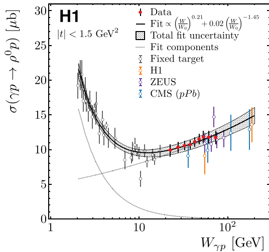
Fig. 11 Elastic ( m_Y=m_\rho ) \rho^0 meson photoproduction cross section \sigma(\gamma p \rightarrow \rho^0 Y) as a function of W_{\gamma p} . The present data are compared to measurements by fixed-target [20–25], HERA [9, 15, 17], and LHC [26] experiments as indicated in the legend. Only total uncertainties are shown. The solid line shows the fit of a sum of two power-law functions to the fixed-target and HERA data. The respective contributions are shown as dotted lines. The fit uncertainty is indicated by a band
