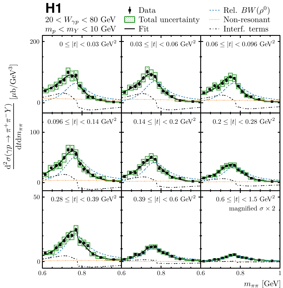
Fig. 13 Proton-dissociative ( m_p < m_Y < 10 GeV) double-differential \pi^+\pi^- photoproduction cross sections d^2\sigma(\gamma p \rightarrow \pi^+\pi^- Y)/dm_{\pi\pi} dt in bins of t and as functions of m_{\pi\pi} . The model that is fitted to the data as described in the text and its components are also shown
