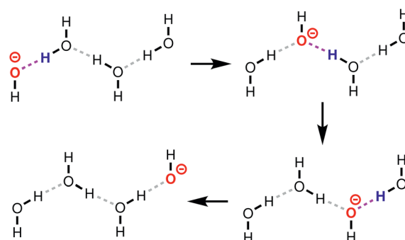
Fig. 1 Schematic representation of the Grotthuss mechanism for the transport of OH^- (red) in water. The protons that participate in the next reaction step are shown in blue, and the hydrogen bond along which they are transferred in magenta. Only the molecules in the water “wire” along which the proton hole diffuses are shown. Each step in the mechanism is aided by fluctuations in the hydrogen bond network with the surrounding water molecules (not shown).
