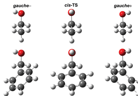
Fig. 2 Comparison between the optimized structures for the gauche – conformers of ethanol and benzyl alcohol as well as the cis transition states (TS) connecting them. While the internal rotations about the C–O and C–C bond are independent from each other in ethanol, they are strongly coupled in benzyl alcohol.
