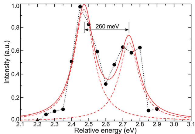
Fig. 5 Dotted line with solid circles: the excitation spectrum obtained as a result of averaging over 7 single SiO 2 nanoparticle excitation spectra. Arbitrary shift of the single particle spectra is indicated by a relative energy axis. The solid red curve shows a fit of two Lorentzian functions to the data. The dashed red curves show the two individual Lorentzian peaks.
