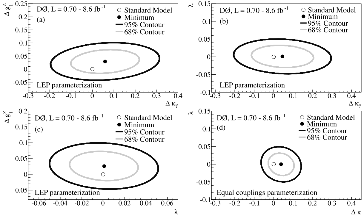
Fig. 4. The 68% and 95% C.L. two-parameter limits on the \gamma WW/ZWW ATGCs \Delta\kappa_\gamma , \Delta\lambda_\gamma and \Delta g_1^Z , assuming the LEP parameterization (a), (b), (c) and on \Delta\kappa and \lambda ATGCs for the equal couplings parameterization (d) with \Lambda = 2 TeV from the combination of WW + WZ \rightarrow \ell\nu jj , WZ \rightarrow \ell\nu\ell\ell , W\gamma \rightarrow \ell\nu\gamma , and WW \rightarrow \ell\nu\ell\nu final states ( \ell = \mu, e ). Black circles indicate the most probable values of ATGCs from the two-parameter fit.
