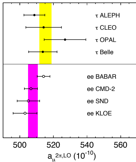
Figure 21.3.5. Evaluation of LO hadronic vacuum polarization contributions to the muon magnetic anomaly in the energy range [2m_\pi, 1.8 \text{ GeV}] from BABAR , other e^+e^- experiments (Davier, Hoecker, Malaescu, Yuan, and Zhang, 2010), and \tau experiments (Davier et al., 2010); see the text for details. The errors include both statistical and systematic sources. For the \tau values, a common systematic error of 1.9 is included to account for uncertainties in the isospin-breaking corrections. The vertical bands represent the combined result, which amount to (507.8 \pm 3.2) \times 10^{-10} for the \pi\pi value, and (515.2 \pm 3.0 \pm 1.9) \times 10^{-10} for the \tau value. They are not obtained as the weighted average of the different values, but originate from a local combination of the respective spectral functions.
