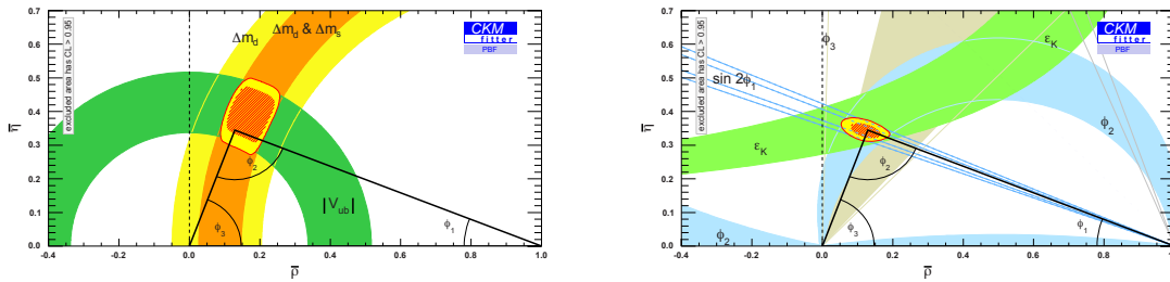
Figure 25.1.2. The consistency between the fit to CP -conserving observables (left) and CP -violating observables (right) from the CKMfit group. The CP -conserving observables are the B^0 - \bar{B}^0 and B_s^0 - \bar{B}_s^0 mass differences, \Delta m_d and \Delta m_s , respectively, and the measurement of |V_{ub}| from semileptonic b \rightarrow d l \nu_l decays. The CP -violating observables are from K ( \varepsilon_K ) and B ( \phi_1, \phi_2, \phi_3 ) decays.
