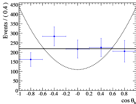
Figure 19.4.4. The helicity angle distribution for \Sigma_c(2455)^0 candidates in B^- \rightarrow \Sigma_c(2455)^0 \bar{p} at BABAR, corrected for efficiency (Aubert, 2008aa). The distributions expected for the spin-1/2 hypothesis (solid, horizontal line) and spin-3/2 hypothesis (dashed curve) are shown. The data are consistent with J = 1/2 and exclude J = 3/2 at the 4\sigma level.
