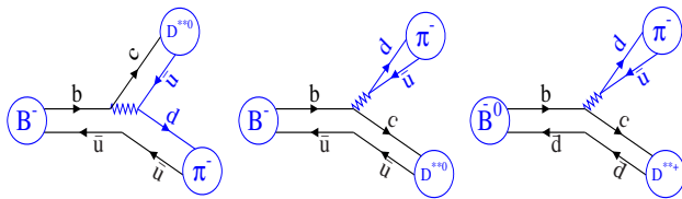
Figure 19.3.2. From (Kuzmin, 2007). Quark-line diagrams for charged (left and middle) and neutral (right) \bar{B} \rightarrow D^{**}\pi decays.
