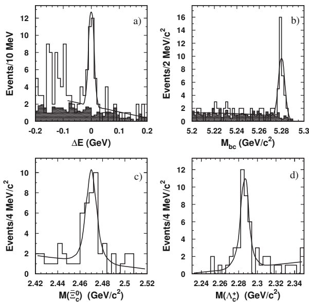
Figure 17.12.4. The \Delta E (a) and m_{ES} = M_{bc} (b) distributions for the B^+ \rightarrow \bar{\Xi}_c^0 \Lambda_c^+ candidates from Belle (Chistov, 2006a). The hatched histograms show the combined \bar{\Xi}_c^0 and \Lambda_c^+ mass sidebands normalized to the signal region. Also shown are the \bar{\Xi}_c^0 (c) and \Lambda_c^+ (d) mass distributions for the B^+ \rightarrow \bar{\Xi}_c^0 \Lambda_c^+ candidates taken from the B signal region of |\Delta E| < 0.025 GeV and m_{ES} > 5.272 GeV/ c^2 . For the \bar{\Xi}_c^0 ( \Lambda_c^+ ) distribution \Lambda_c^+ ( \bar{\Xi}_c^0 ) is required to be within \pm 15 MeV/ c^2 of the nominal mass. The overlaid curves are the fit results.
