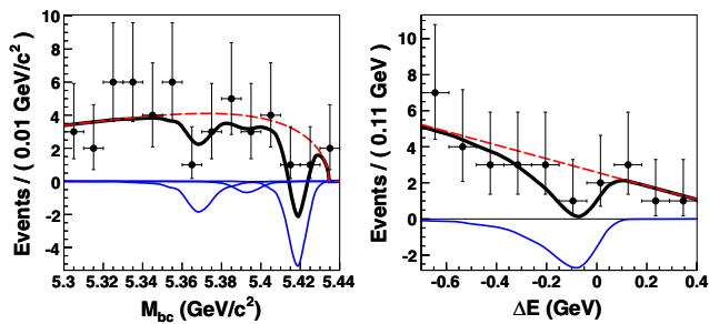
Figure 17.11.5. m_{\text{ES}} (left; called M_{\text{bc}} on the plot) and \Delta E (right) data yield (points) and fit results for B_s^0 \rightarrow \gamma\gamma in the Belle analysis (Wicht, 2008). The solid black curve represents the overall fit, while the dashed red and solid blue curves represent the continuum/combinatorial background and signal components of the fit, respectively. See Chapter 23 for an explanation of the structure of the m_{\text{ES}} distribution. On the \Delta E projection, m_{\text{ES}} > 5.4 \text{ GeV}/c^2 is required to select only the B_s^* \bar{B}_s^* contributions from \Upsilon(5S) . The fit returns a slight negative yield, consistent with zero within the data statistical uncertainties.
