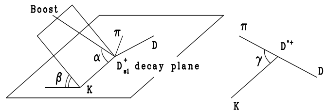
Figure 19.3.27. Definitions of the angles: \alpha is the D_{s1}(2536) helicity angle measured in the D_{s1}(2536) CM frame as the angle between the boost direction in the e^+e^- CM frame and the K_S^0 momentum; \beta is the angle between the plane formed by these two vectors and the D_{s1}(2536) decay plane measured also in the D_{s1}(2536) rest frame; \gamma is the D^{*+} helicity angle between the \pi^+ and K_S^0 momenta in the D^{*+} rest frame.
