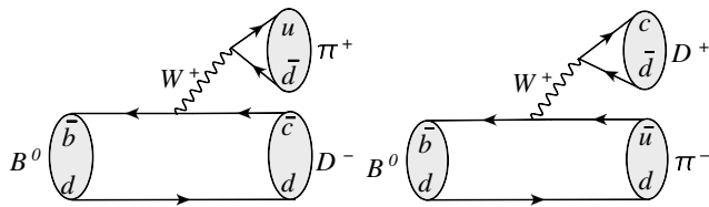
Figure 17.8.12. Typical leading order Feynman diagrams for the CF decay B^0 \rightarrow D^- h^+ (left) and the DCS decay B^0 \rightarrow D^+ h^- (right).
