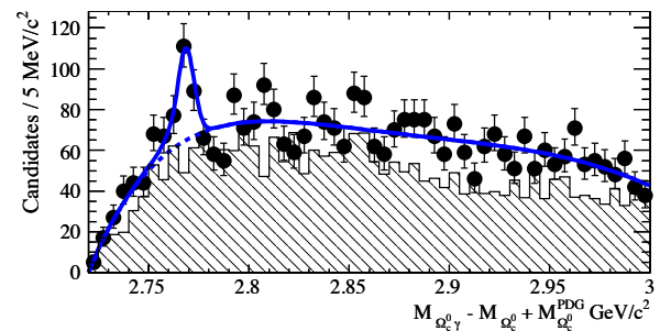
Figure 19.4.7. The m(\Omega_c^0\gamma) invariant mass spectrum at BABAR , combining four decay modes of the \Omega_c : \Omega^-\pi^+ , \Omega^-\pi^+\pi^0 , \Omega^-\pi^+\pi^-\pi^+ , \Xi^-K^-\pi^+\pi^+ . The \Omega_c^* resonance is visible. The shaded histogram represents the combinatoric background estimated from the \Omega_c^0 mass sidebands. (Aubert, 2006ah)
