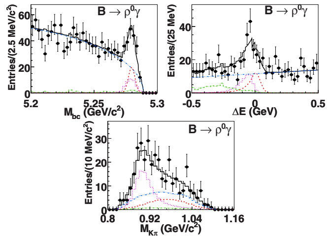
Figure 17.9.8. From (Taniguchi, 2008). Signal for B^0 \rightarrow \rho^0\gamma from Belle in m_{ES} ( =M_{bc} ), \Delta E and M(K\pi) (dashed, red) and backgrounds from B^0 \rightarrow K^{*0}\gamma (dotted, magenta), other B decays (dot-dashed, green) and continuum (dot-dot-dashed, cyan). Each spectrum is made with signal-region cuts on the other plotted quantities.
