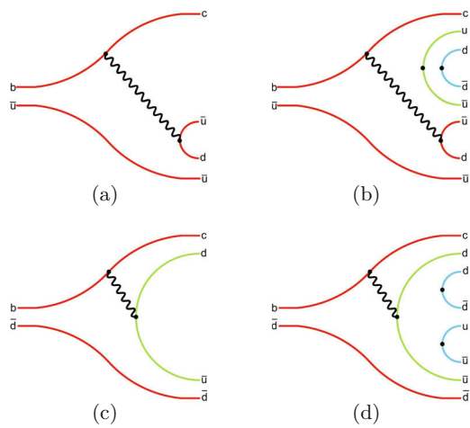
Figure 17.12.13. Spectator diagrams of type 2, illustrating the basic picture for a \mathfrak{B}_1\mathfrak{B}_2 threshold enhancement: (b) shows one diagram for B^- \rightarrow \Lambda_c^+ p \pi^- with preferentially low \mathfrak{B}_1\mathfrak{B}_2 mass related to the meson pair diagram (a), and (d) shows \bar{B}^0 \rightarrow \Sigma_c^0 p \pi^+ with preferentially high \mathfrak{B}_1\mathfrak{B}_2 mass related to the diquark pair diagram (c).
