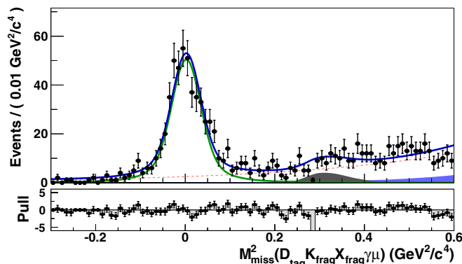
Figure 19.1.40. From (Zupanc, 2013b). M_{\text{recoil}}^2(H_c K X \gamma \mu^-) spectrum for D_s^+ \rightarrow \mu^+ \nu_\mu candidates for the selected data (points with error bars). The solid green line shows the contribution of signal, the red dashed line the contribution of combinatorial background, while the contributions of D_s^+ \rightarrow \tau^+ \nu_\tau and D_s^+ \rightarrow \bar{K}^0 K^+ or \eta \pi^+ are indicated by the full blue and dark gray histograms, respectively.
