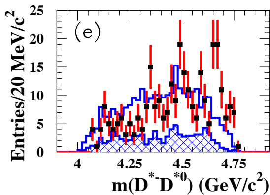
Figure 18.3.13. The D^{*0}D^{*-} invariant mass spectrum from B \rightarrow D^{*0}D^{*-}K decays from BABAR (Aubert, 2003f). The hatched histograms show the contribution expected from the combinatorial background. The open histograms show the contribution expected for the three-body decay generated with a phase-space model.
