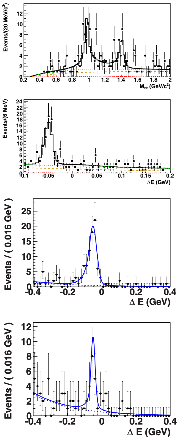
Figure 23.3.8. Data fit projections for B_s^0 \rightarrow J/\psi \pi^+ \pi^- (top two plots), B_s^0 \rightarrow J/\psi \eta ( \eta \rightarrow \gamma\gamma ) and B_s^0 \rightarrow J/\psi \eta' ( \eta' \rightarrow \rho\gamma ) (bottom two plots, respectively). The J/\psi \pi^+ \pi^- M_{\pi\pi} ( \Delta E ) distributions are for events in the \Delta E ( f_0(980) ) signal region. The J/\psi \eta^{(\prime)} \Delta E distributions are for events in the m_{ES} signal region. The dotted curves show the total background contribution. Plots are from Li (2011, 2012).
