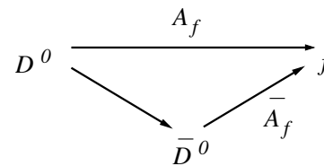
Figure 19.2.3. Illustration of interference between direct D meson decays and decays through mixing into the final state f , accessible to either D^0 or \bar{D}^0 .
