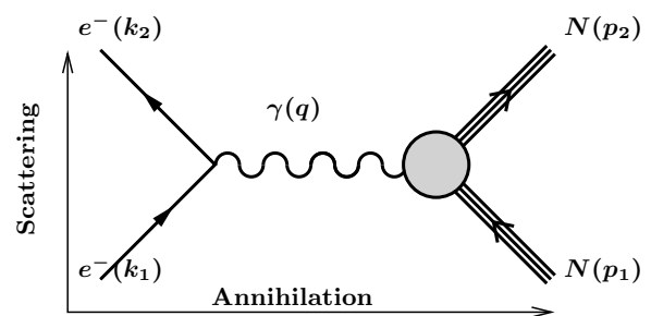
Figure 21.3.18. One-photon exchange Feynman diagram for scattering e^-N \rightarrow e^-N and annihilation e^+e^- \rightarrow N\bar{N} .
