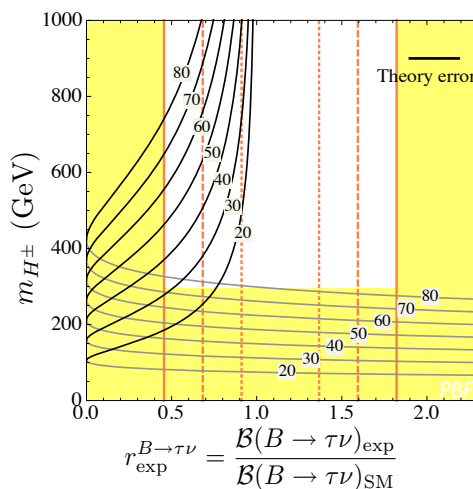
Figure 25.2.3. Constraints on the charged Higgs mass in the Type II 2HDM from the B Factory measurements of \mathcal{B}(B \rightarrow \tau\nu) and \mathcal{B}(B \rightarrow X_s\gamma) . The x -axis represents the present experimental value of \mathcal{B}(B \rightarrow \tau\nu) normalized to the SM prediction (see text for details). The vertical yellow regions are excluded by the current world average experimental value, \mathcal{B}(B \rightarrow \tau\nu)_{\text{exp}} = (1.15 \pm 0.23) \times 10^{-6} , at 95% C.L., while the 1\sigma, 2\sigma, 3\sigma errors on the same experimental value are denoted by the dotted, dashed, and solid lines, respectively. The horizontal yellow region is excluded by the \mathcal{B}(B \rightarrow X_s\gamma) measurement (see Eq. 25.2.9). The grey and the black lines correspond to the predictions of the Type II 2HDM given in Eq. (25.2.12), respectively, with labels denoting the different values of \tan\beta .
