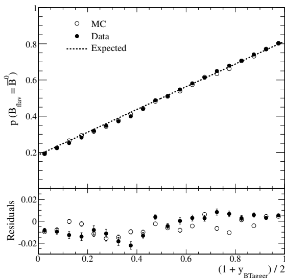
Figure 8.6.3. Probability of observing a fully reconstructed \bar{B}^0 on the B_{\text{flav}} side as a function of the probability p_{B_{\text{tag}}=B^0} = (1 + y_{B_{\text{Tagger}}})/2 of having a B^0 on the B_{\text{tag}} side. The dotted line shows the dependence expected for a perfectly trained tagging algorithm. The solid points are from the full BABAR B_{\text{flav}} control sample, the open circles are obtained from simulation. A contribution of up to 22% from combinatorial background is subtracted in each bin based on a fit to the m_{\text{ES}} distribution. The residuals with respect to the expectation are shown at the bottom.
