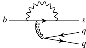
Figure 17.6.4. Penguin diagram of b \rightarrow q\bar{q}s .
