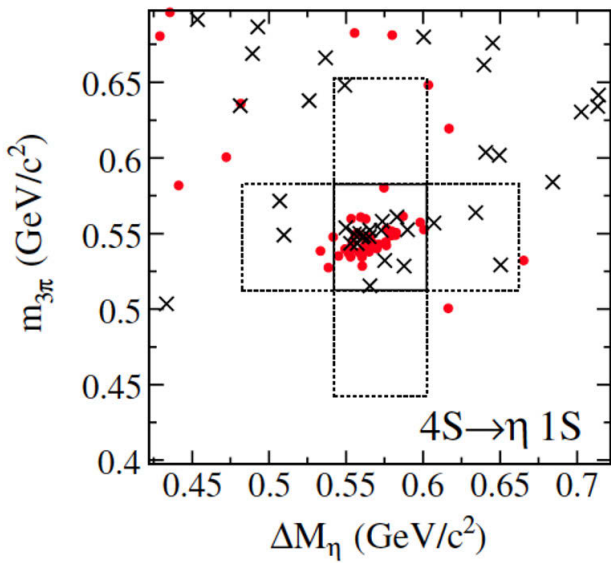
Figure 18.4.20. The distribution of M_{3\pi} vs \Delta M_{\eta} = M_{3\pi\mu} - M_{ll} for \eta\Upsilon(1S) candidate events, demonstrating the observed signal (Aubert, 2008bc). Solid lines delimit the signal region, while dashed lines delimit the sideband regions used for the background estimate. Crosses represent the data from the \Upsilon(1S) \rightarrow e^+e^- sample and dots the data from the \Upsilon(1S) \rightarrow \mu^+\mu^- sample.
