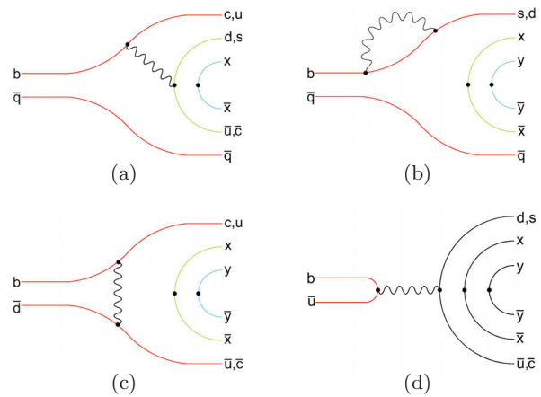
Figure 17.12.5. Quark diagrams for two-body baryonic B decay \bar{B} \rightarrow \mathfrak{B}_1 \mathfrak{B}_2 . The wavyline represents a W , while gluon lines are omitted. Quark antiquark pairs from the vacuum are denoted as x, y and determine the flavor of the two final baryons. In this and subsequent figures, the colors of the quark lines are significant: see the discussion in Section 17.12.2.2.
