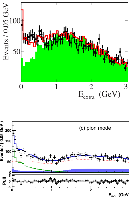
Figure 19.1.41. E_{\text{extra}} ( E_{\text{ECL}} in case of Belle) distribution for D_s^- \rightarrow \tau^- \bar{\nu}_\tau, \tau^- \rightarrow e^- \nu_\tau \bar{\nu}_e (del Amo Sanchez, 2010g) (top) and for D_s^- \rightarrow \tau^- \bar{\nu}_\tau, \tau^- \rightarrow \pi^- \nu_\tau (Zupanc, 2013b). The points represent the data with statistical error bars. In the top plot the open histogram is from the fit, and the solid histogram is the background component from the fit. For the bottom plot the lines represent different components of the fit.
