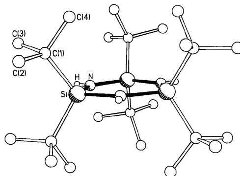
Fig. 1. The molecular structure, showing the atom-numbering scheme. tert -Butyl H atoms are omitted.
