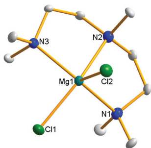
Fig. 3 Molecular structure of one of the independent molecules of complex 5 [MgCl 2 ·PMDETA]. All ellipsoids are displayed at 50% probability and H atoms have been omitted for clarity. Selected bond parameters (Å/°): Mg1–Cl1, 2.3913(7) [2.3770(6)]; Mg1–Cl2, 2.3108(7) [2.3371(6)]; Mg1–N1, 2.1932(15) [2.1886(13)]; Mg1–N2, 2.3230(13) [2.2959(13)]; Mg1–N3, 2.2142(15) [2.2226(13)]; Cl1–Mg1–Cl2, 106.26(3) [105.26(3)]; Cl1–Mg1–N1, 93.44(4) [93.19(4)]; Cl2–Mg1–N1, 109.78(4) [106.25(4)]; Cl1–Mg1–N2, 156.89(4) [156.78(4)]; Cl2–Mg1–N2, 96.84(4) [98.09(4)]; Cl1–Mg1–N3, 93.20(4) [92.27(4)]; Cl2–Mg1–N3, 109.25(4) [113.79(4)]; N1–Mg1–N2, 78.91(5) [79.78(5)]; N1–Mg1–N3, 136.63(5) [136.49(5)]; N2–Mg1–N3, 78.42(5) [78.48(5)]. Bond parameters of second independent molecule are in parentheses.
