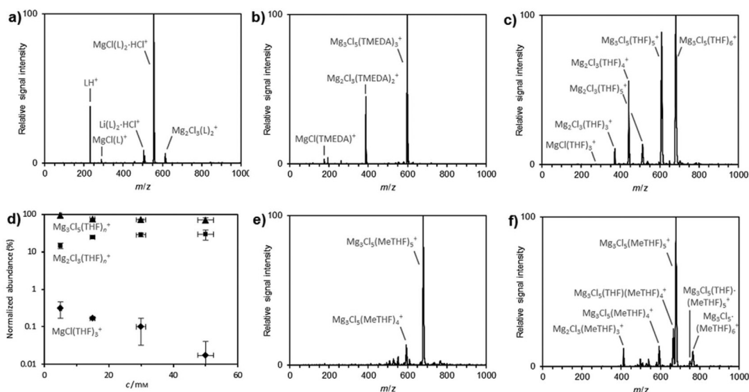
Fig. 5 (a) positive-ion mode ESI mass spectrum of a 20 mM solution of [(\text{Dipp})(\text{Me}_3\text{Si})\text{NALCl}_3]^- [\text{MgCl}\cdot\text{Me}_6\text{TREN}]^+ ( 2 ) in THF ( \text{L} = \text{Me}_6\text{TREN} ); (b) positive-ion mode ESI mass spectrum of a saturated solution ( c \leq 10 mM) of [(\text{Dipp})(\text{Me}_3\text{Si})\text{NALCl}_3]^- [\text{Mg}_3(\mu_3\text{-Cl})_2(\mu_2\text{-Cl})_3\cdot 3\text{TMEDA}]^+ ( 3 ) in THF; (c) positive-ion mode ESI mass spectrum of a 20 mM solution of [(\text{Dipp})(\text{Me}_3\text{Si})\text{NALCl}_3]^- [\text{Mg}_2(\mu_2\text{-Cl})_3\cdot 6\text{THF}]^+ ( 1 ) in THF; (d) concentration dependence of the normalized abundances of mono-, di-, and trinuclear cations observed upon positive-ion mode ESI of solutions of ( 1 ) in THF; (e) positive-ion mode ESI mass spectrum of a 20 mM solution of [(\text{Dipp})(\text{Me}_3\text{Si})\text{NALCl}_3]^- [\text{Mg}_3(\mu_3\text{-Cl})_2(\mu_2\text{-Cl})_3\cdot 6\text{MeTHF}]^+ ( 4 ) in MeTHF; (f) positive-ion mode ESI mass spectrum of a 20 mM solution of ( 1 ) in MeTHF.
