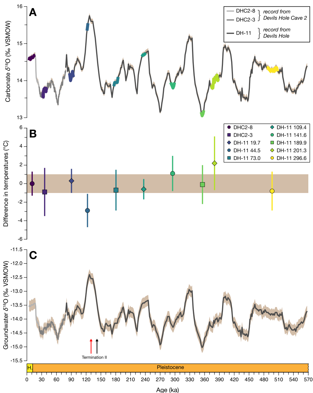
Figure 3. Dual clumped isotope thermometry reveals stable calcite precipitation temperatures in the Devils Hole caves. (a) Carbonate \delta^{18}\text{O} record from Devils Hole and Devils Hole Cave 2 (Winograd et al., 2006). The colored sections correspond to the age range of the samples in this study (Table 1). The range of the \delta^{18}\text{O}_{\text{cc}} values in the sampled intervals is less than 0.35\text{‰} . The analytical uncertainty of the \delta^{18}\text{O}_{\text{cc}} measurements is \pm 0.07\text{‰} (shaded area). (b) Differences in the \Delta_{47} -derived calcite precipitation temperatures (Petersen et al., 2019) between DHC2-8 ( 33.7^\circ\text{C} ) and older samples. The shaded area encloses the 95% confidence interval of the mean \Delta_{47} ( \text{CDES90} ) value of all samples, which corresponds to \pm 1^\circ\text{C} . Error bars represent the 95% confidence intervals of the measurements. (c) Groundwater \delta^{18}\text{O} values, reconstructed using the \delta^{18}\text{O}_{\text{cc}} values from panel A and 33.7 (\pm 1)^\circ\text{C} (Coplen, 2007). The timing of Termination II, that is, the penultimate glacial/interglacial transition, occurs at 142 ka in Devils Hole \delta^{18}\text{O}_{\text{cc}} record (black arrow) (Winograd et al., 2006) and at 130 ka in the LR04 benthic \delta^{18}\text{O} stack (red arrow) (Lisiecki & Raymo, 2005).
