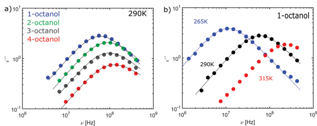
Fig. 8 (a) Loss spectra of n -octanol ( n = 1,2,3,4) measured at a temperature of 290 K, (b) loss spectrum of 1-octanol at temperatures of 265 K (blue), 290 K (black) and 315 K (red). The solid lines reflect fits using the Cole–Davidson function.
