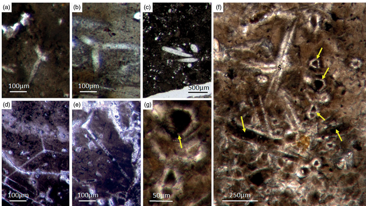
Fig. 5. (Colour online) Basic demosponge spicules. (a, b, d) Various types of four-rayed spicules with an angle of about 120^\circ between the rays (Fon31, 59, 11). (c) Group of thick monaxon-style spicules (Fon11). (e) Typical triaene (orthotriaene) spicule (Fon11). (f, g) Aggregates of spicules (S) with possible remains of enlarged axial filament structure (arrows). Axial canal filled with organic matter (kerogen) and exhibiting hexagonal cross-sections as known from demosponges (Fon10).
