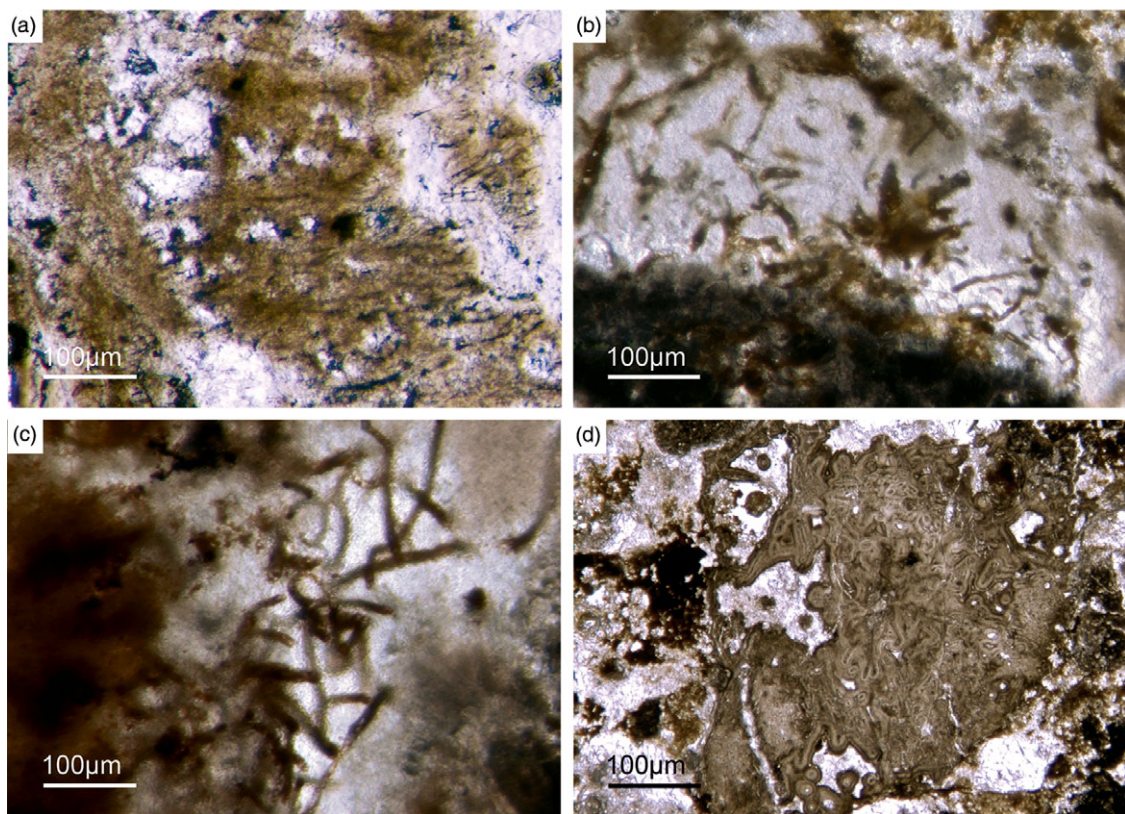
Fig. 15. (Colour online) Filamentous microbial remains. (a) Long filamentous structures, probably remains of sulphide-oxidizing bacteria (SOX-B) (Fon35). (b) Filamentous remains within bright phosphorite (Fon36). (c) Network of large filaments interpreted as remains of SOX-B (Fon36). (d) Sponge skeleton that is strongly cemented by multilayered phosphate, probably resulting from intense flow of P-rich fluids.
