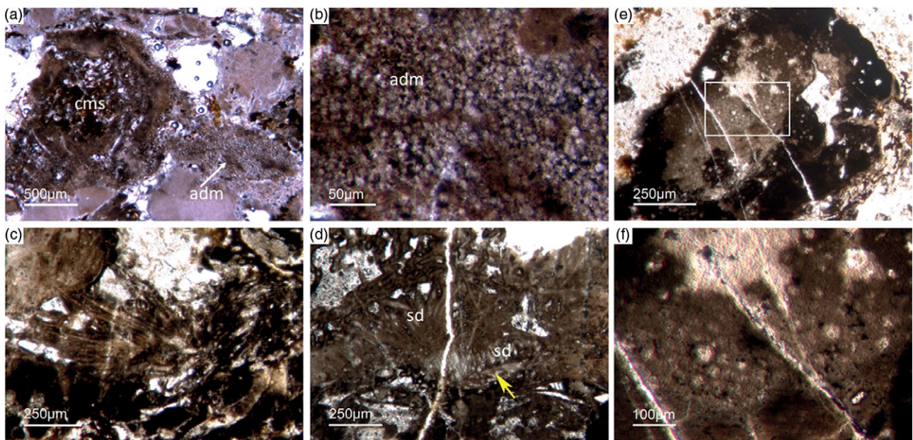
Fig. 7. (Colour online) Articulated demosponge spicular skeletons. (a, b) Representing a 'hadromerid' skeleton. The sponge shows a dense crust of putative asterose dermal microscleres (adm) and randomly orientated choanosomal, probably monaxon spicules (cms) (Fon 38). (c) Radially orientated long styles typical for various early Cambrian sponges like Choia , Choiaella , Hamptoniella (Fon20). (d) Plumose arrangement of short dermal styles (ds) and tangentially arranged monaxons (arrow) on the outer part of the skeleton (Fon20). (e, f) The fossil represents asterose microscleres characteristic for chondrillid hadromerids ((f) enlarged area of (e)) (Fon17).
